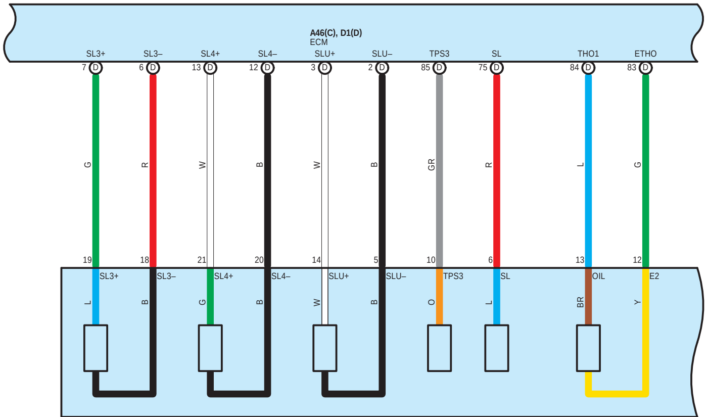
D57 ECT Solenoid (Transmission Wire)
