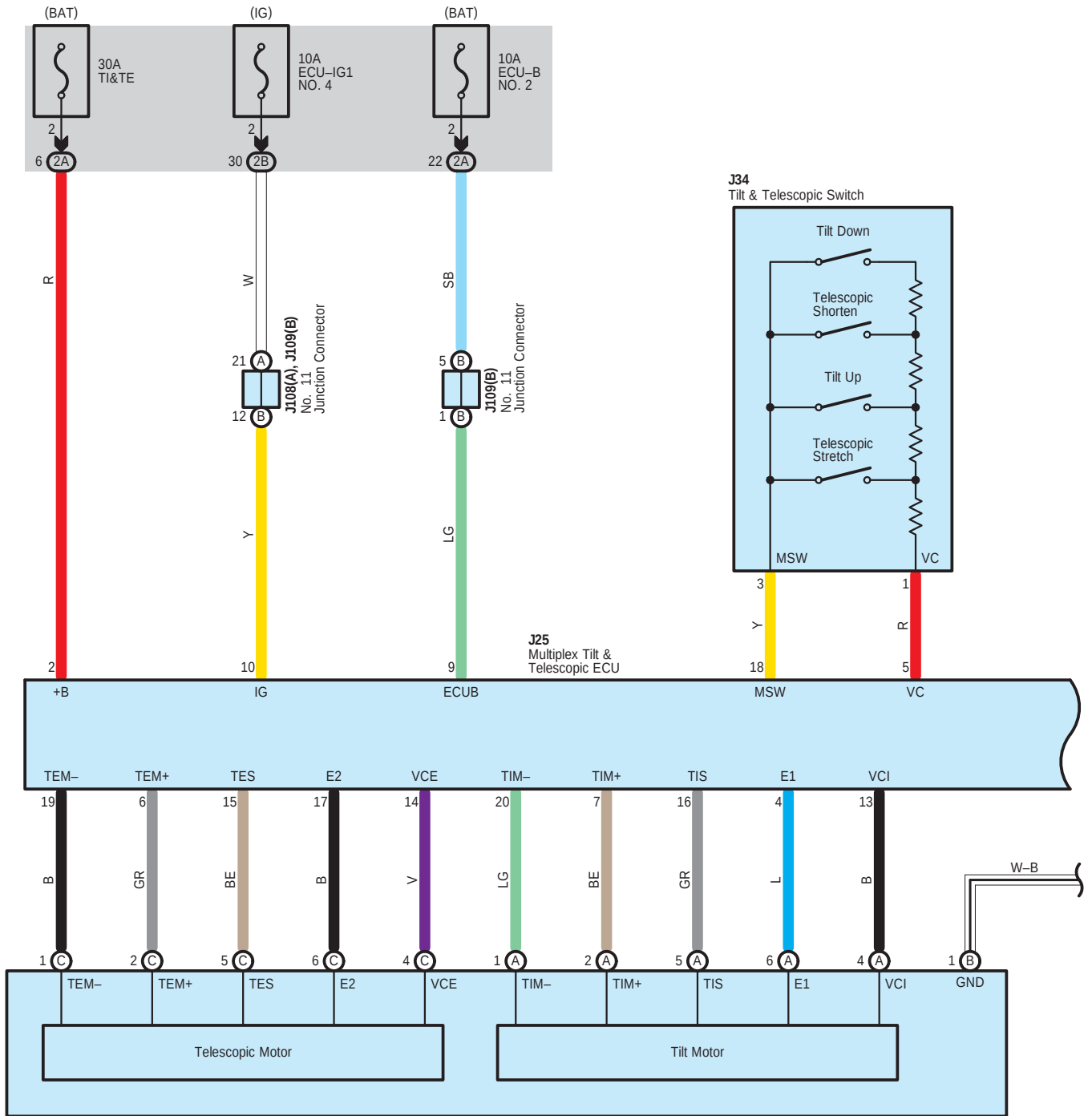
J24(A), J27(B), J69(C) Electric Power Steering Column Sub-Assembly
