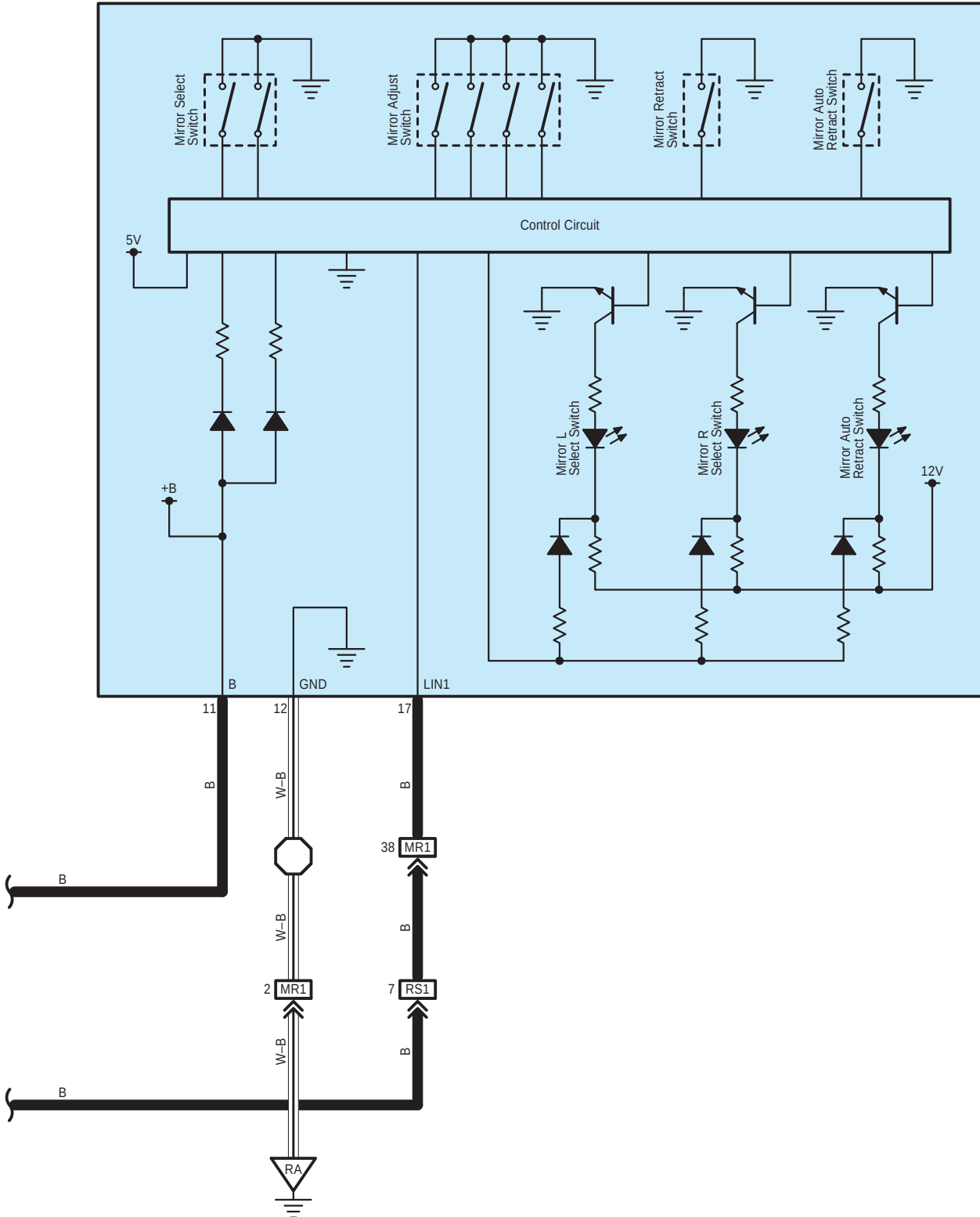
M7 Multiplex Network Master Switch Assembly
