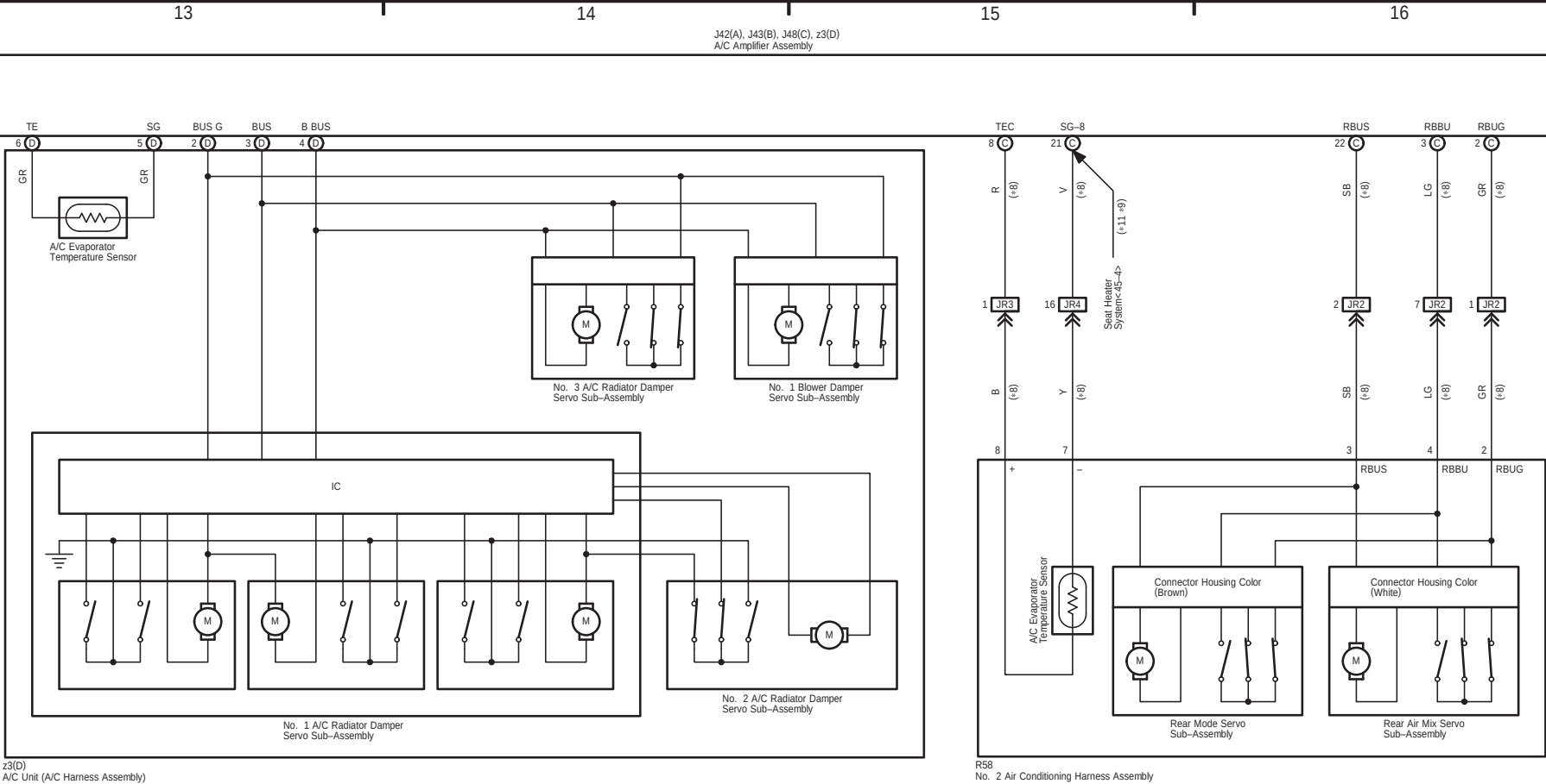
z3(D) A/C Unit (A/C Harness Assembly)
