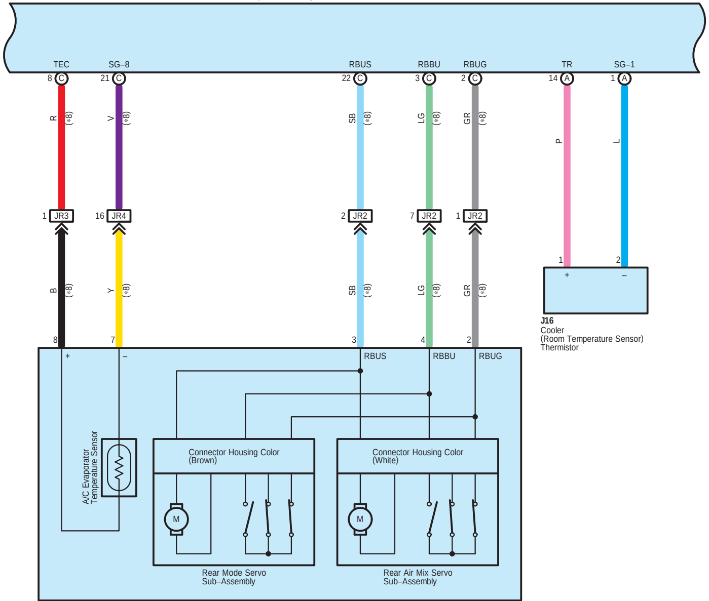
R58 No. 2 Air Conditioning Harness Assembly
