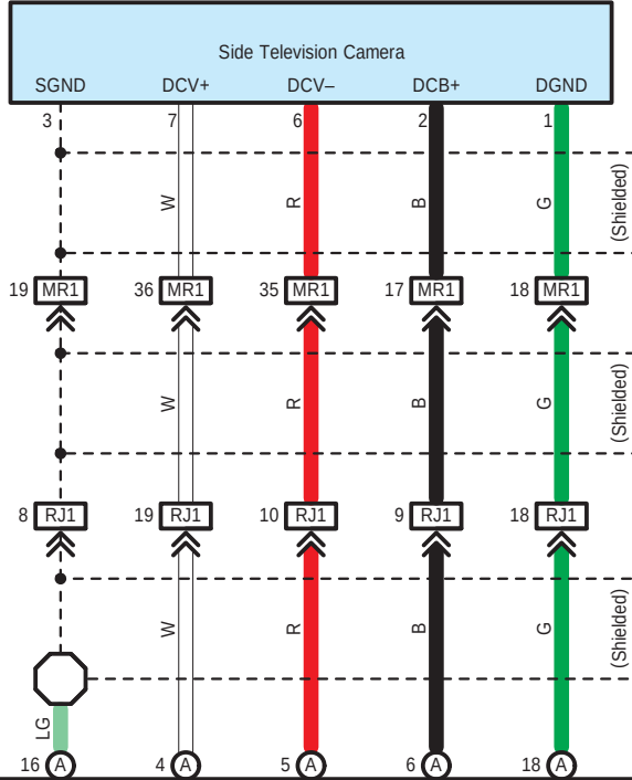
M1 Outer Rear View Mirror Assembly RH
