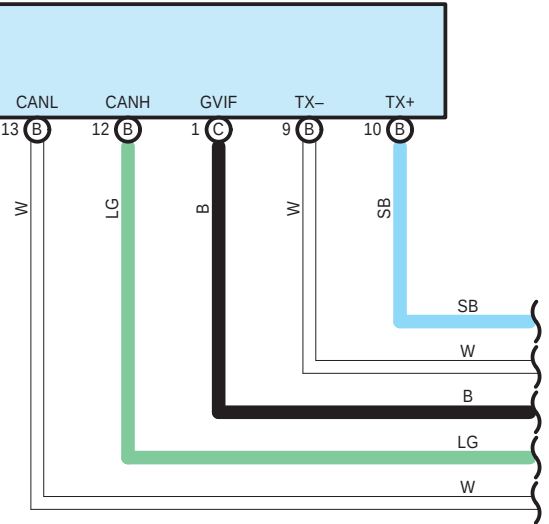
J72(A), J73(B), J135(C) Parking Assist ECU
