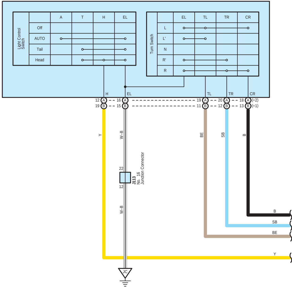
J28(A), (B) Headlight Dimmer Switch Assembly
