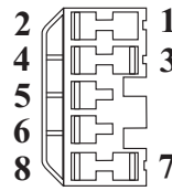
Internal Transaxle Harness "Female" Coupler Connector Number "CO8"
