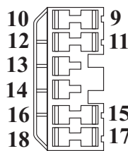
Internal Transmission Harness "Female" Coupler Connector Number "JB10a"
