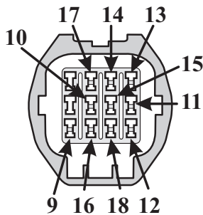
External Transaxle Harness Connector Number "H2-03"
