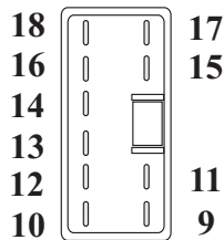
Internal Transaxle Harness "Male" Coupler Connector Number "CO10"
