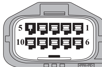
View Looking Into Vehicle Harness Connector JB156
