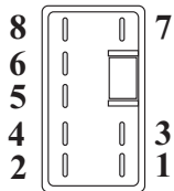
Internal Transmission Harness "Male" Coupler Connector Number "JB8"
