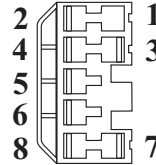
Internal Transaxle Harness "Female" Coupler Connector Number "H2-07"
