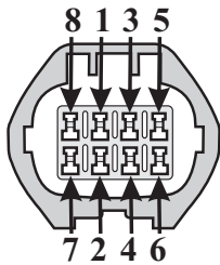
External Transaxle Harness Connector Number "H2-06"
