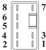
External Transaxle Connector Number "H1-05"
