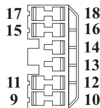
View Looking Into The Internal Transaxle Harness "Female" Coupler Connector Number "T10"
