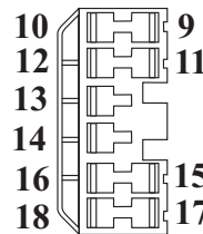
Internal Transaxle Harness "Female" Coupler Connector Number "H2-04"
