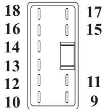
Internal Transmission Harness "Male" Coupler Connector Number "JB10"
