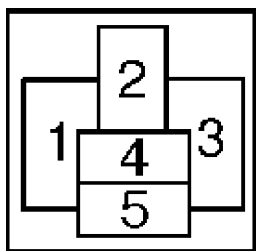
Fig. 2: Identifying Defogger Relay Terminals (Diamante, Eclipse, Galant, Mirage & Montero Sport)
