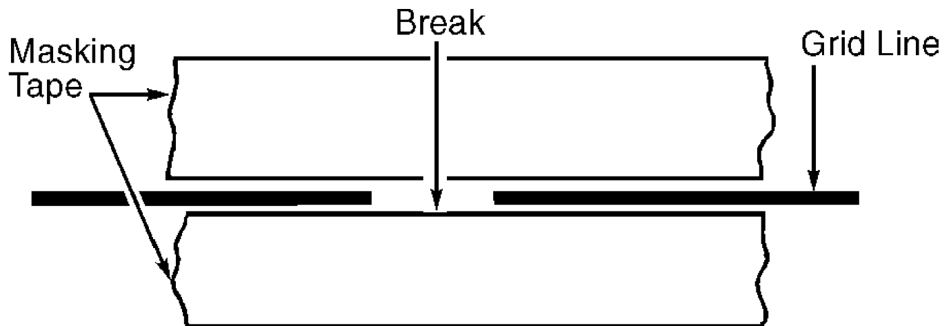
Fig. 8: Repairing Rear Defogger Grid Element
