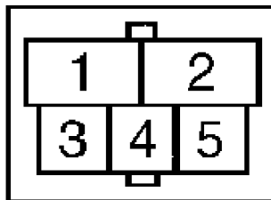
Fig. 3: Identifying Defogger Relay Terminals (Montero) Courtesy of Mitsubishi Motor Sales of America
