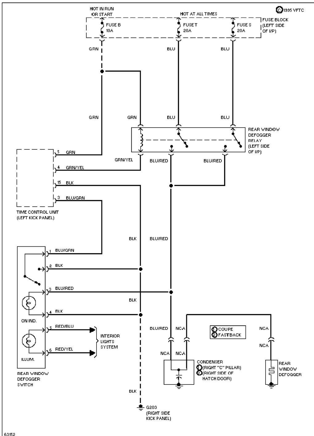
Defogger Circuit
