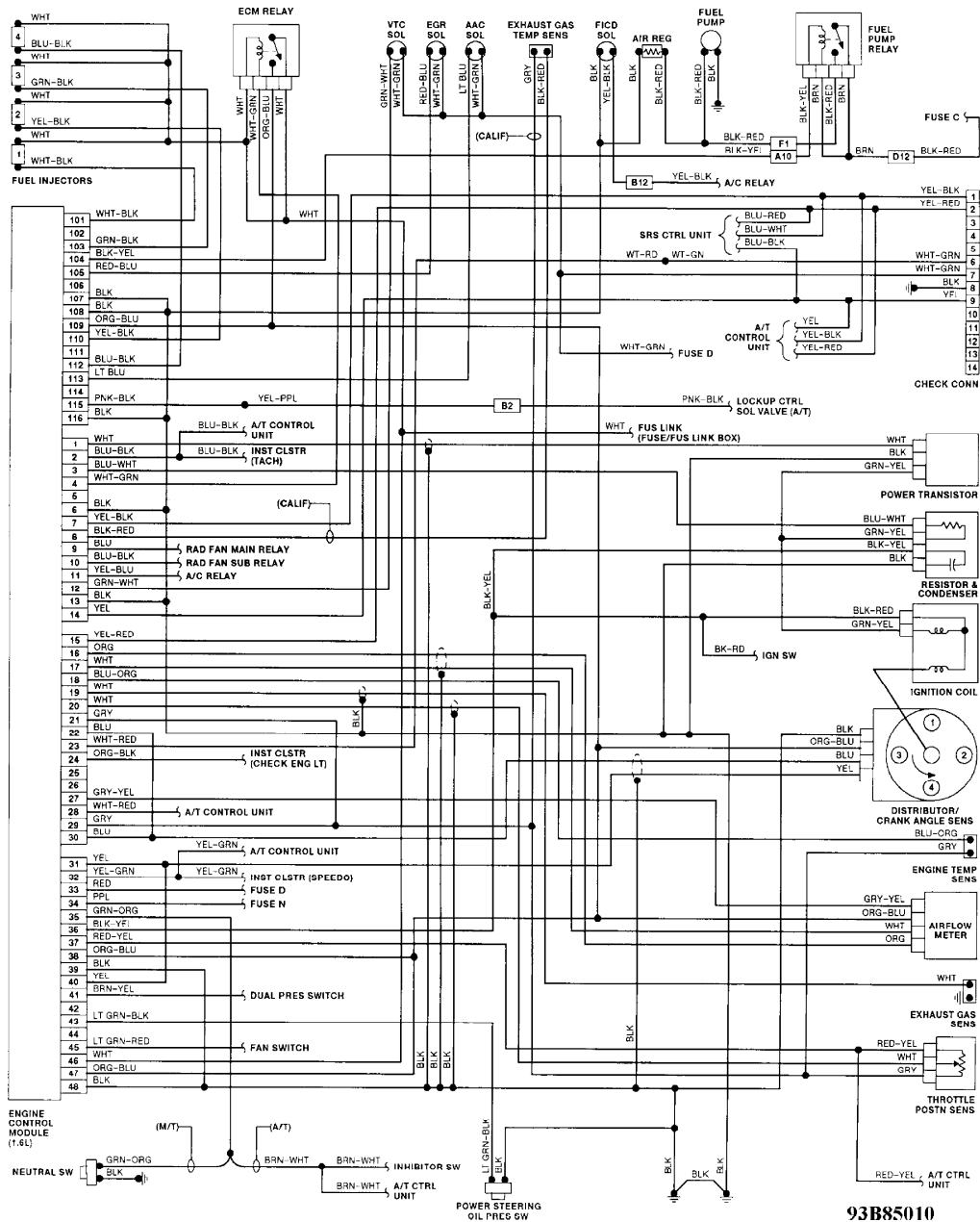
Fig. 1: Wiring Diagram (NX & Sentra 1.6L)
