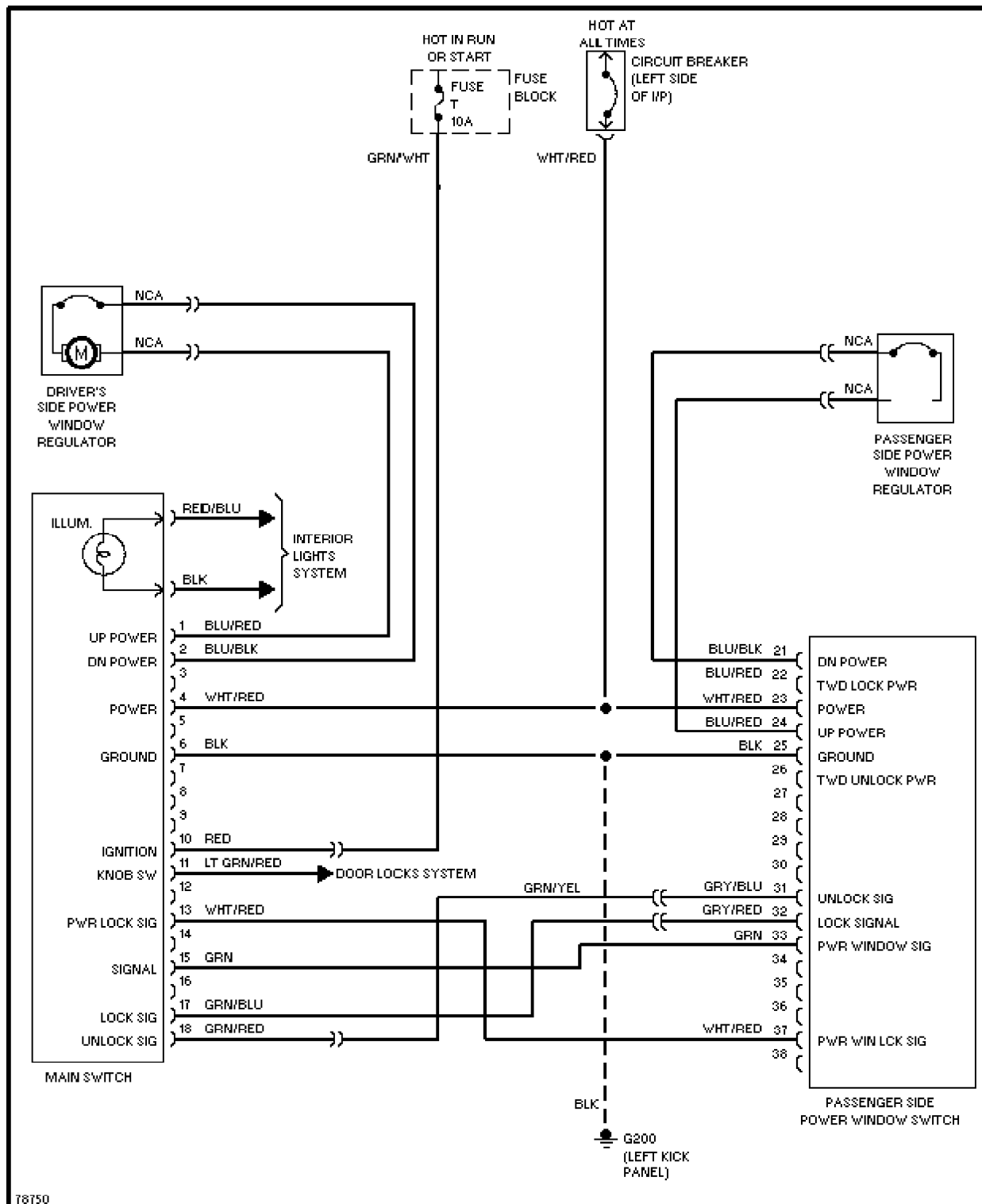
Power Window Circuit, Coupe
