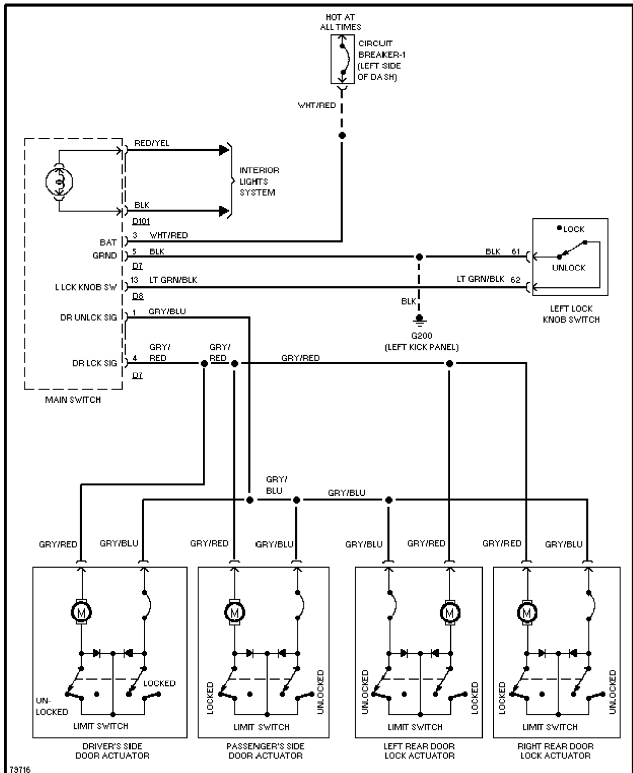
Power Door Lock Circuit, Sedan
