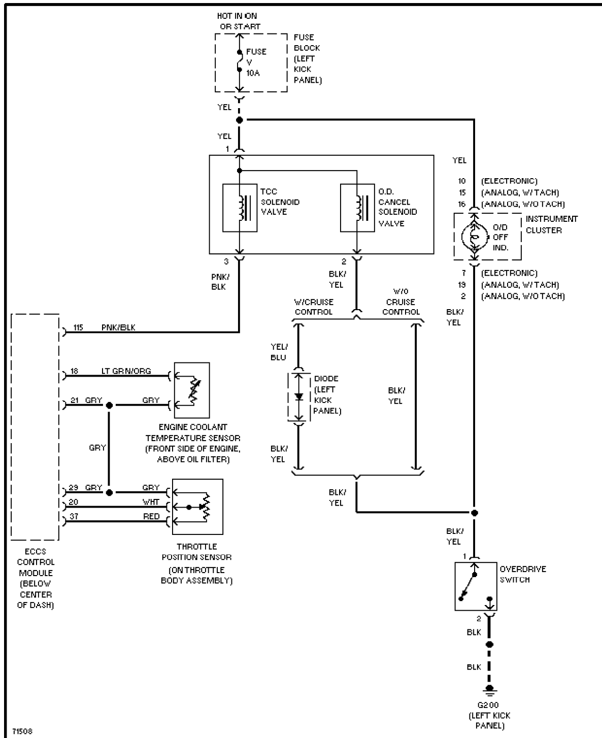
1.6L, Transmission Circuit
