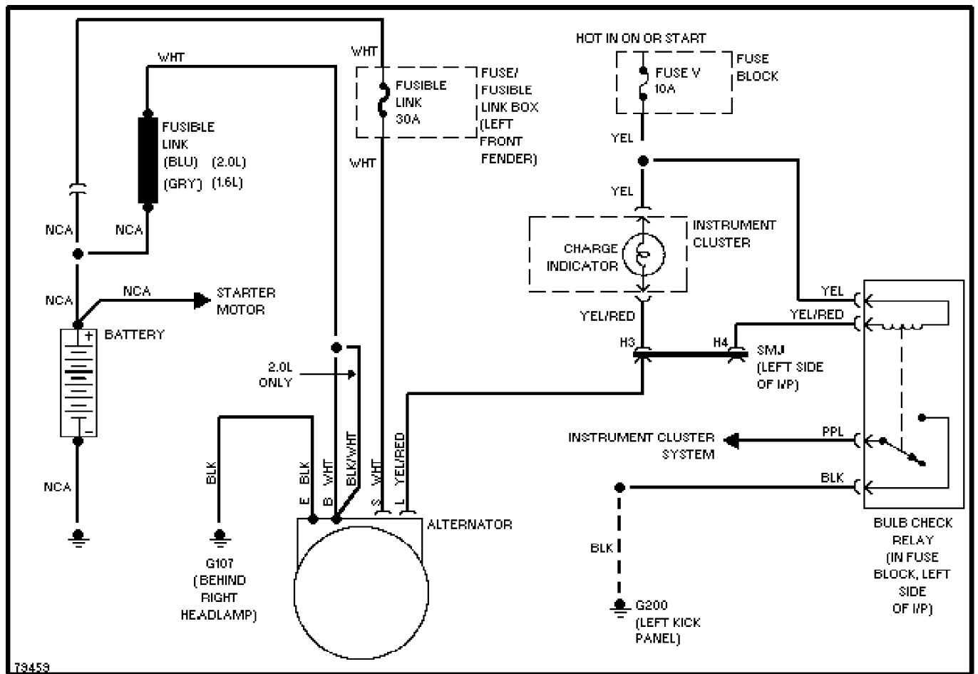
Charging Circuit
