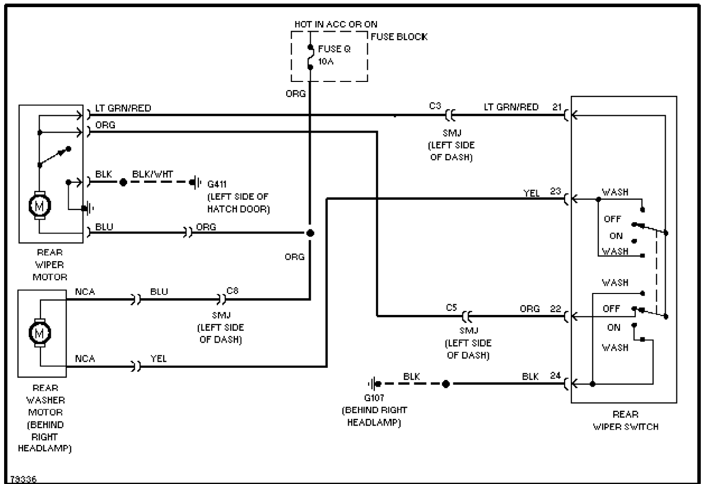
Rear Washer/Wiper Circuit
