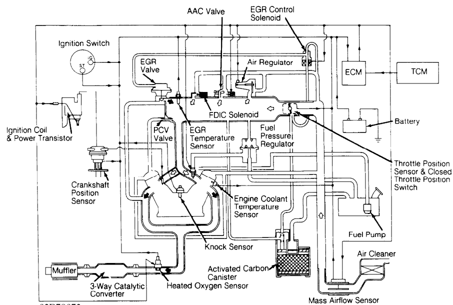
Fig. 9: Vacuum Diagram (Quest) Courtesy of Nissan Motor Co., U.S.A.
