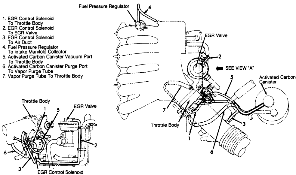
Fig. 7: Vacuum Diagram (Pickup - 4-Cylinder) Courtesy of Nissan Motor Co., U.S.A.
