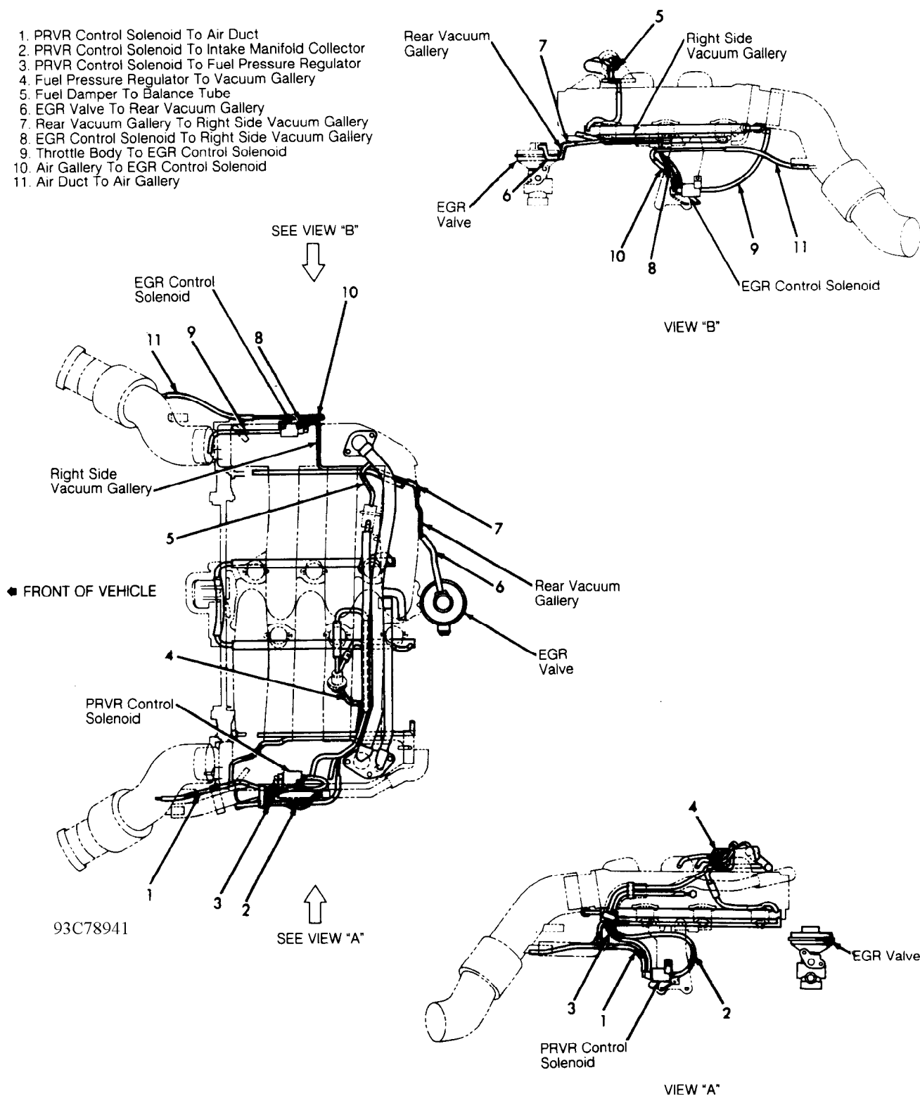
Fig. 12: Vacuum Diagram (300ZX Non-Turbo) Courtesy of Nissan Motor Co., U.S.A.
