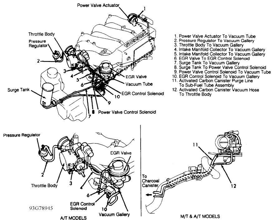
Fig. 4: Vacuum Diagram (Maxima - VE30DE) Courtesy of Nissan Motor Co., U.S.A.
