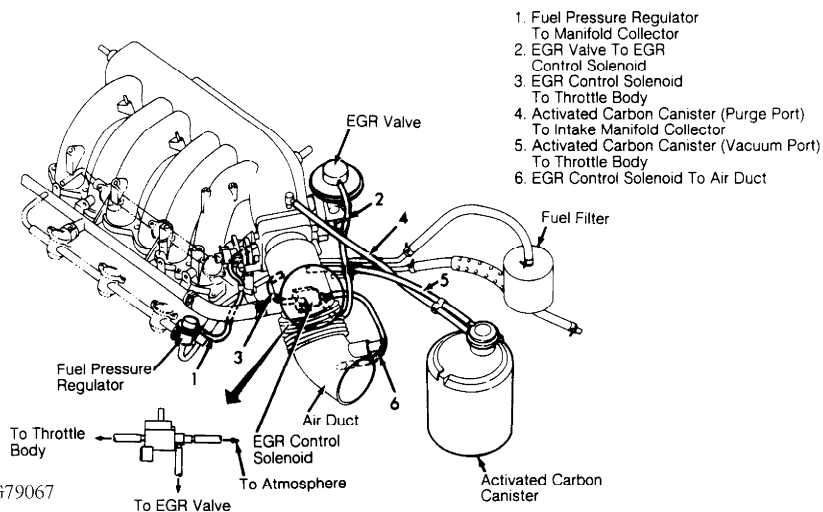
Fig. 10: View Of EGR System Components (Quest) Courtesy of Nissan Motor Co., U.S.A.
