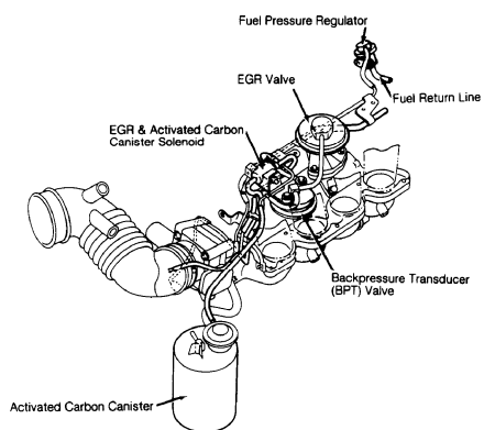
Fig. 2: View Of EGR System Components (Altima) Courtesy of Nissan Motor Co., U.S.A.
