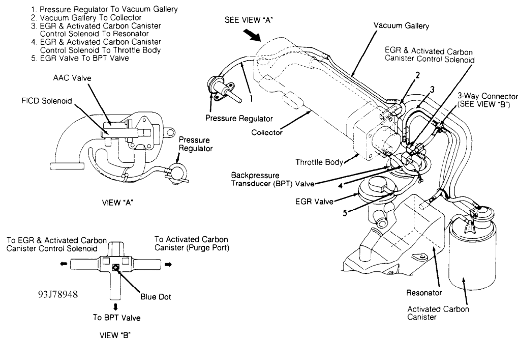
93J78948 Fig. 6: Vacuum Diagram (NX & Sentra - 2.0L) Courtesy of Nissan Motor Co., U.S.A.
