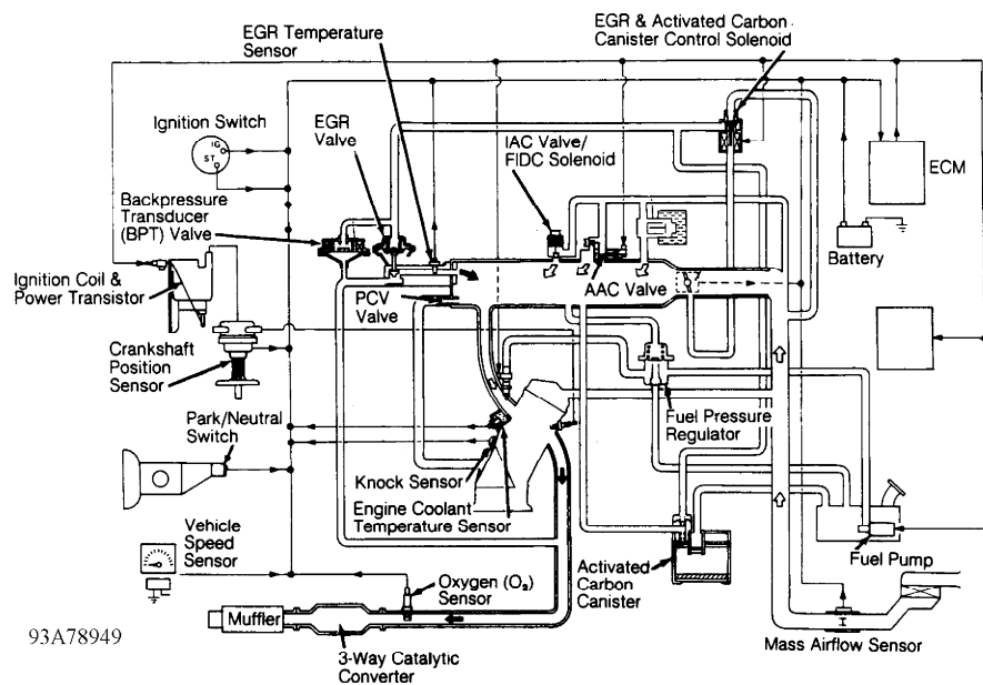
Fig. 1: Vacuum Diagram (Altima) Courtesy of Nissan Motor Co., U.S.A.
