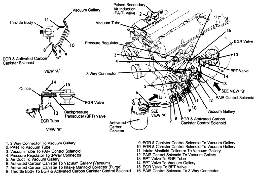
93J78947 Fig. 5: Vacuum Diagram (NX & Sentra - 1.6L) Courtesy of Nissan Motor Co., U.S.A.
