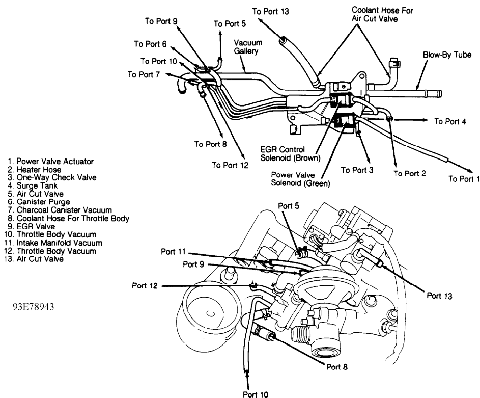
Fig. 3: Vacuum Diagram (Maxima - VG30E) Courtesy of Nissan Motor Co., U.S.A.
