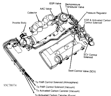
Fig. 11: Vacuum Diagram (240SX) Courtesy of Nissan Motor Co., U.S.A.
