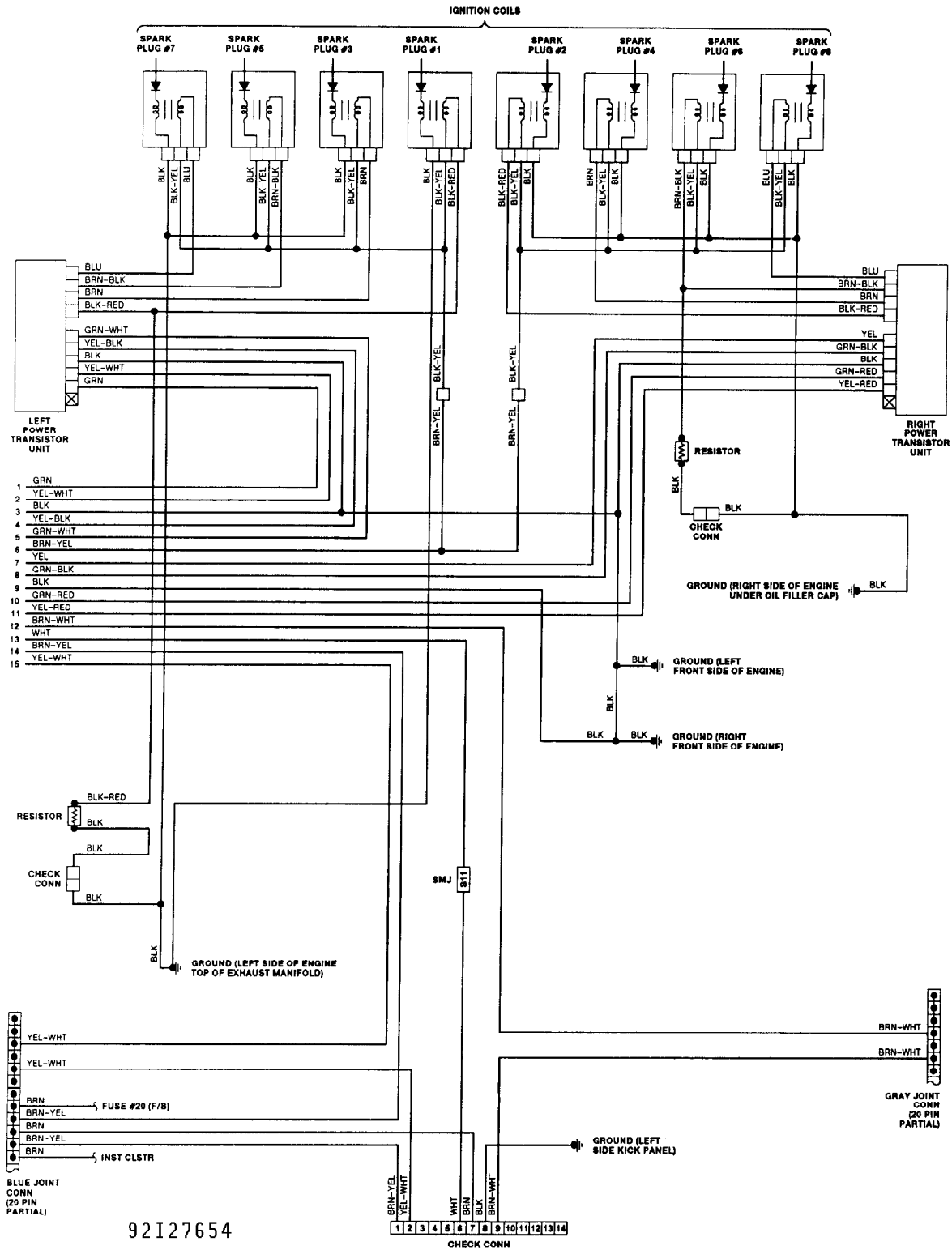
Fig. 7: Wiring Diagram (Q45 4.5L - 3 Of 3)
