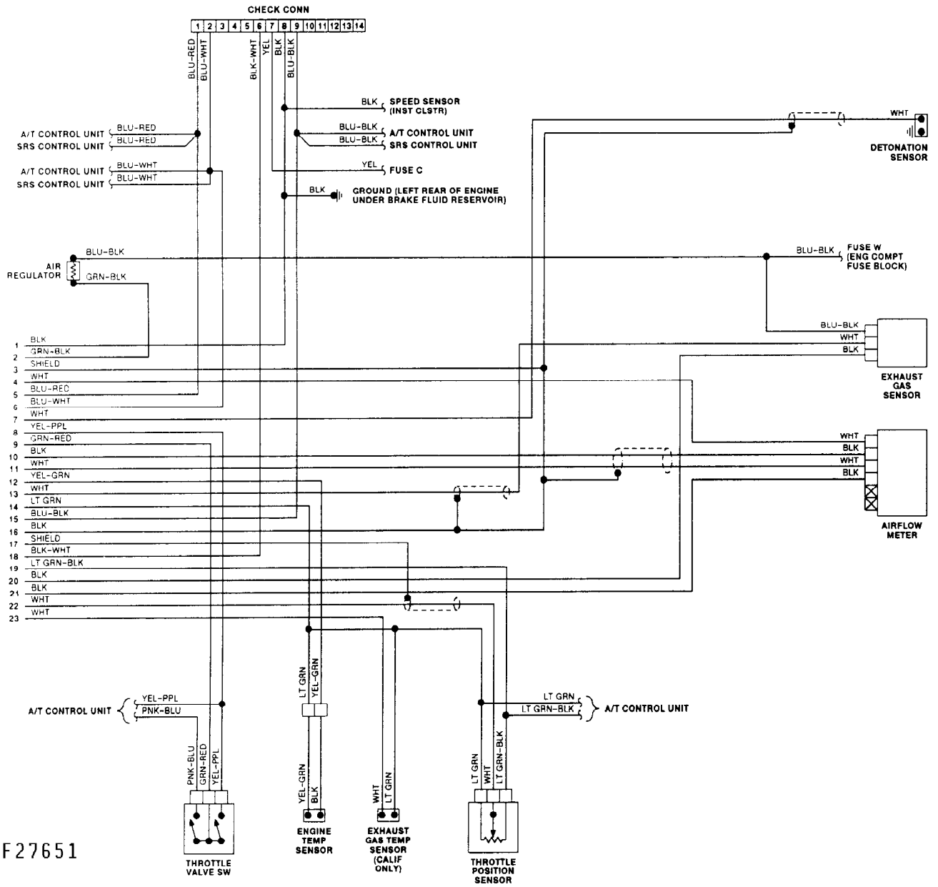
Fig. 4: Wiring Diagram (M30 3.0L - 2 Of 2)
