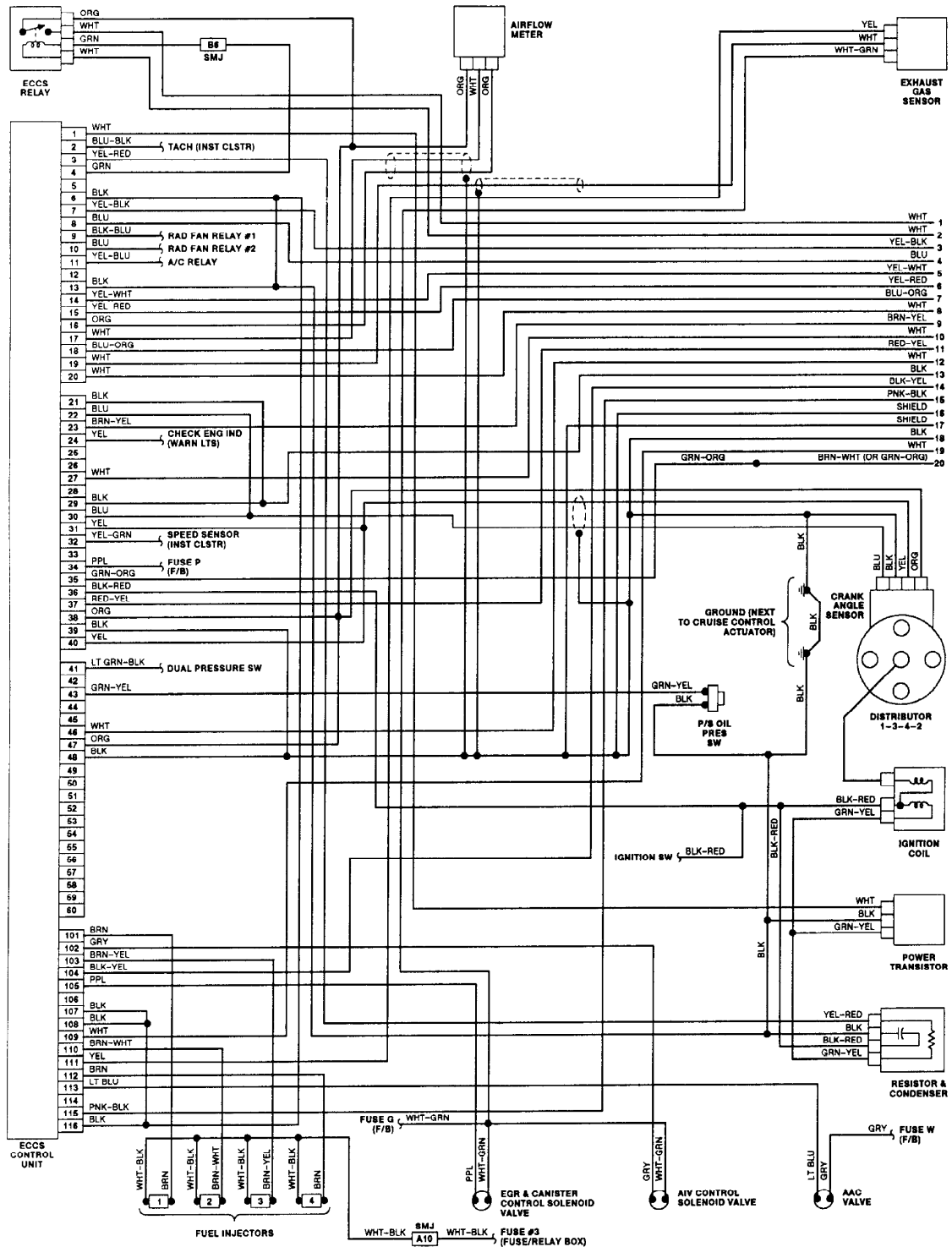
Fig. 1: Wiring Diagram (G20 2.0L - 1 Of 2)
