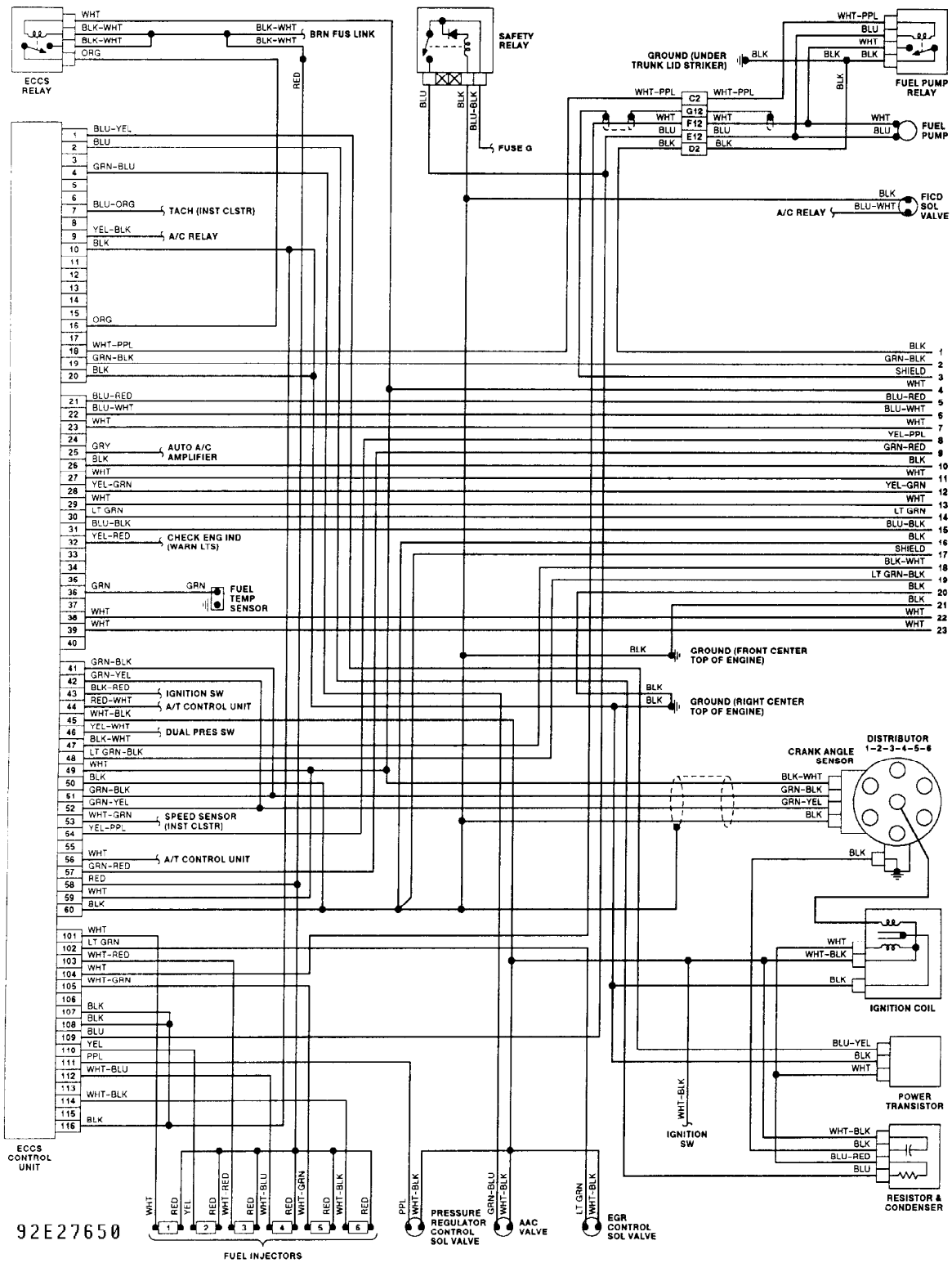
Fig. 3: Wiring Diagram (M30 3.0L - 1 Of 2)
