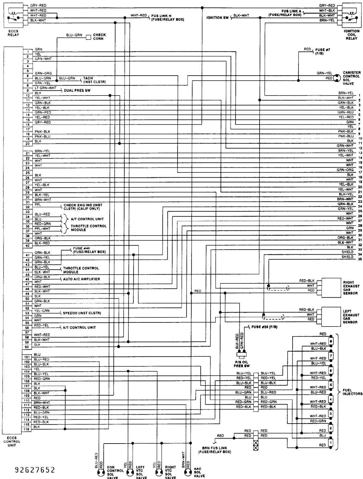
Fig. 5: Wiring Diagram (Q45 4.5L - 1 Of 3)
