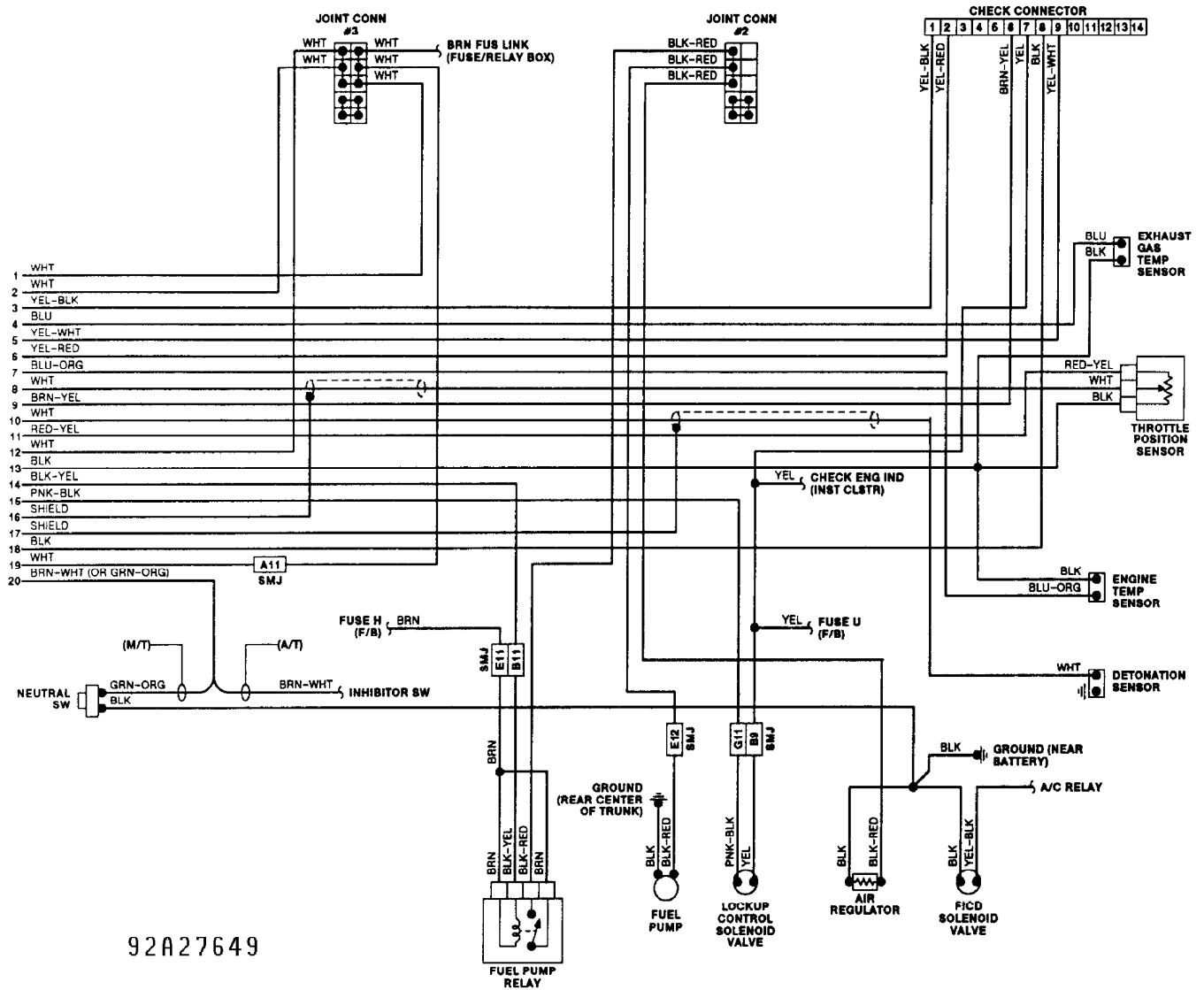
Fig. 2: Wiring Diagram (G20 2.0L - 2 Of 2)
