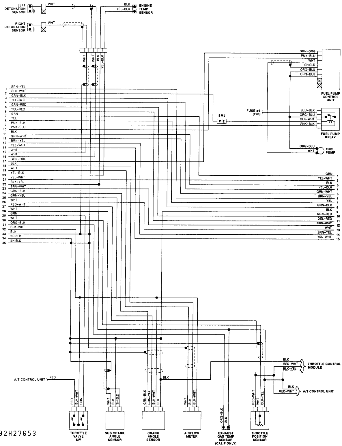
Fig. 6: Wiring Diagram (Q45 4.5L - 2 Of 3)
