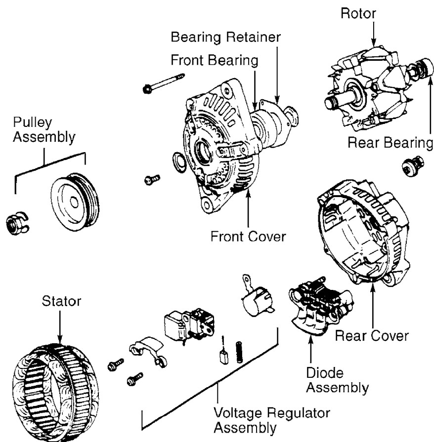
Fig. 2: Exploded View of Mitsubishi Alternator Courtesy of Nissan Motor Co., U.S.A.
