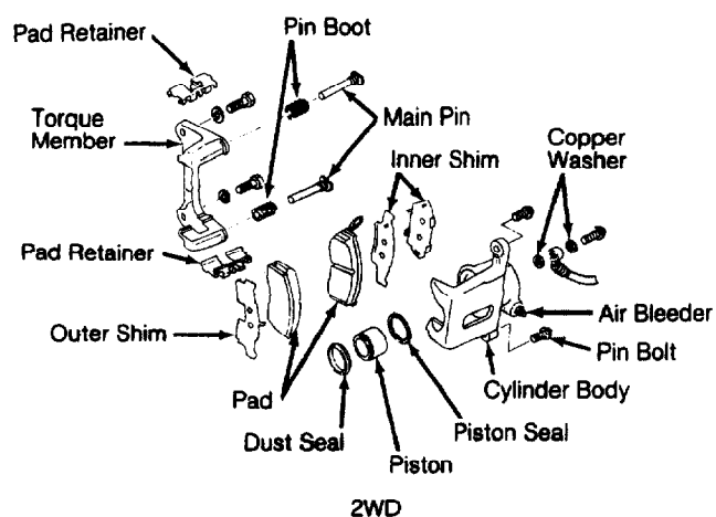
Fig. 8: Exploded View of Front Brakes (Sentra) Courtesy of Nissan Motor Co., U.S.A.
