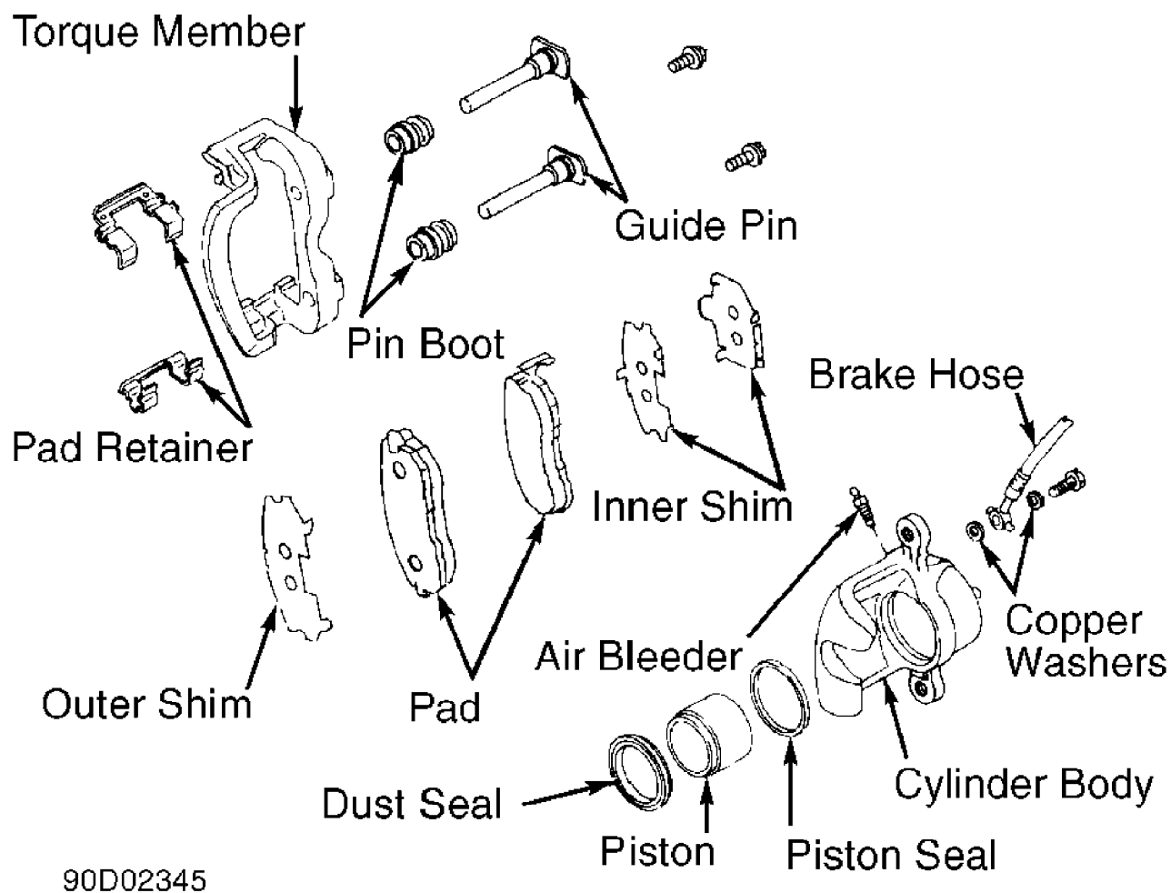
Fig. 6: Exploded View of Front Brakes (Axxess & Maxima) Courtesy of Nissan Motor Co., U.S.A.
