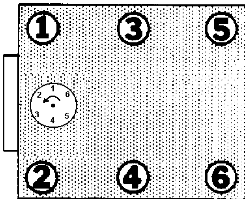
FIRING ORDER 1-2-3-4-5-6
