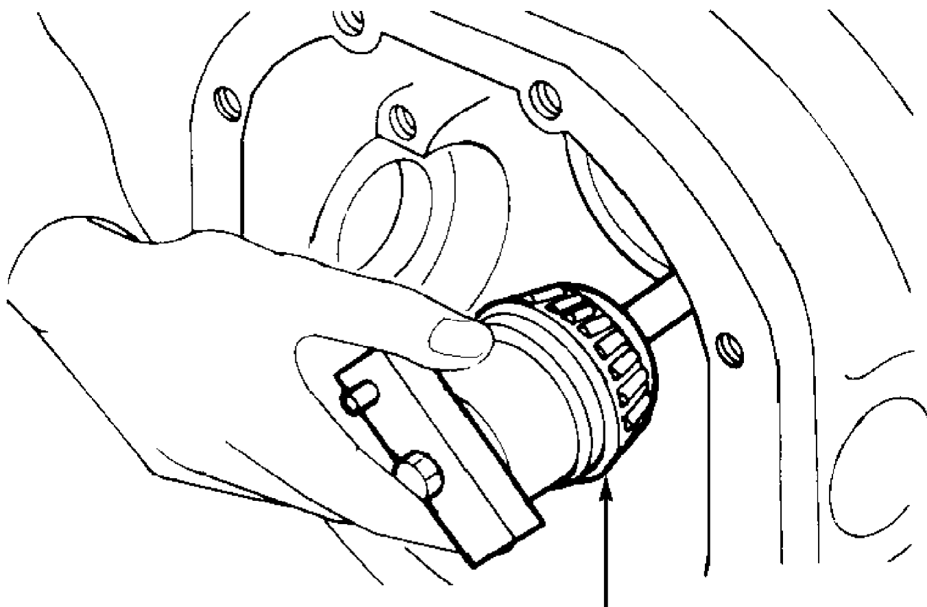
Fig. 5: Installing Rear Pinion Bearing and Preload Shim Selector Assembly Courtesy of Nissan Motor Co., U.S.A.
