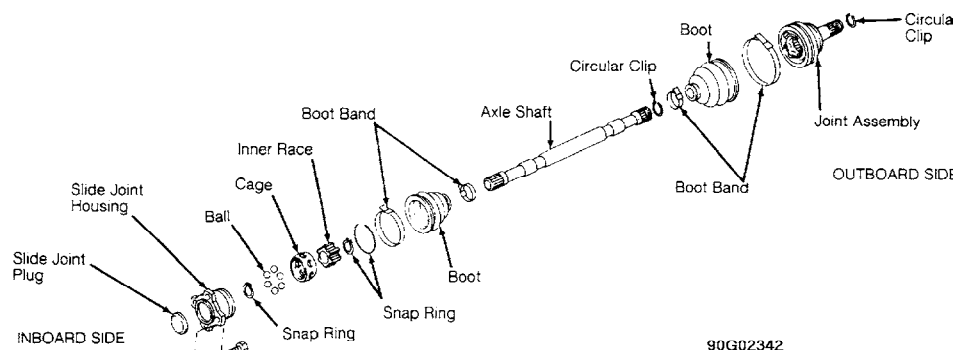
Fig. 2: Exploded View of 300ZX Drive Shaft Courtesy of Nissan Motor Co., U.S.A.
