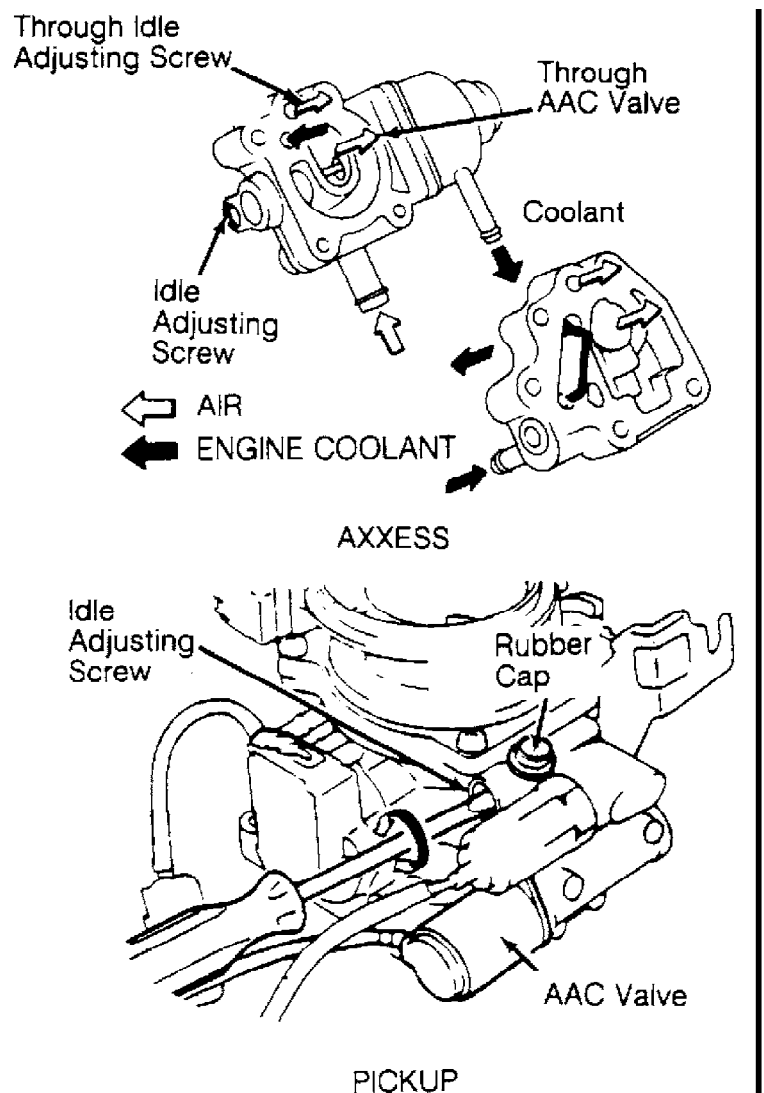
Fig. 2: Adjusting Idle Speed (Axxess) Courtesy of Nissan Motor Co., U.S.A.
