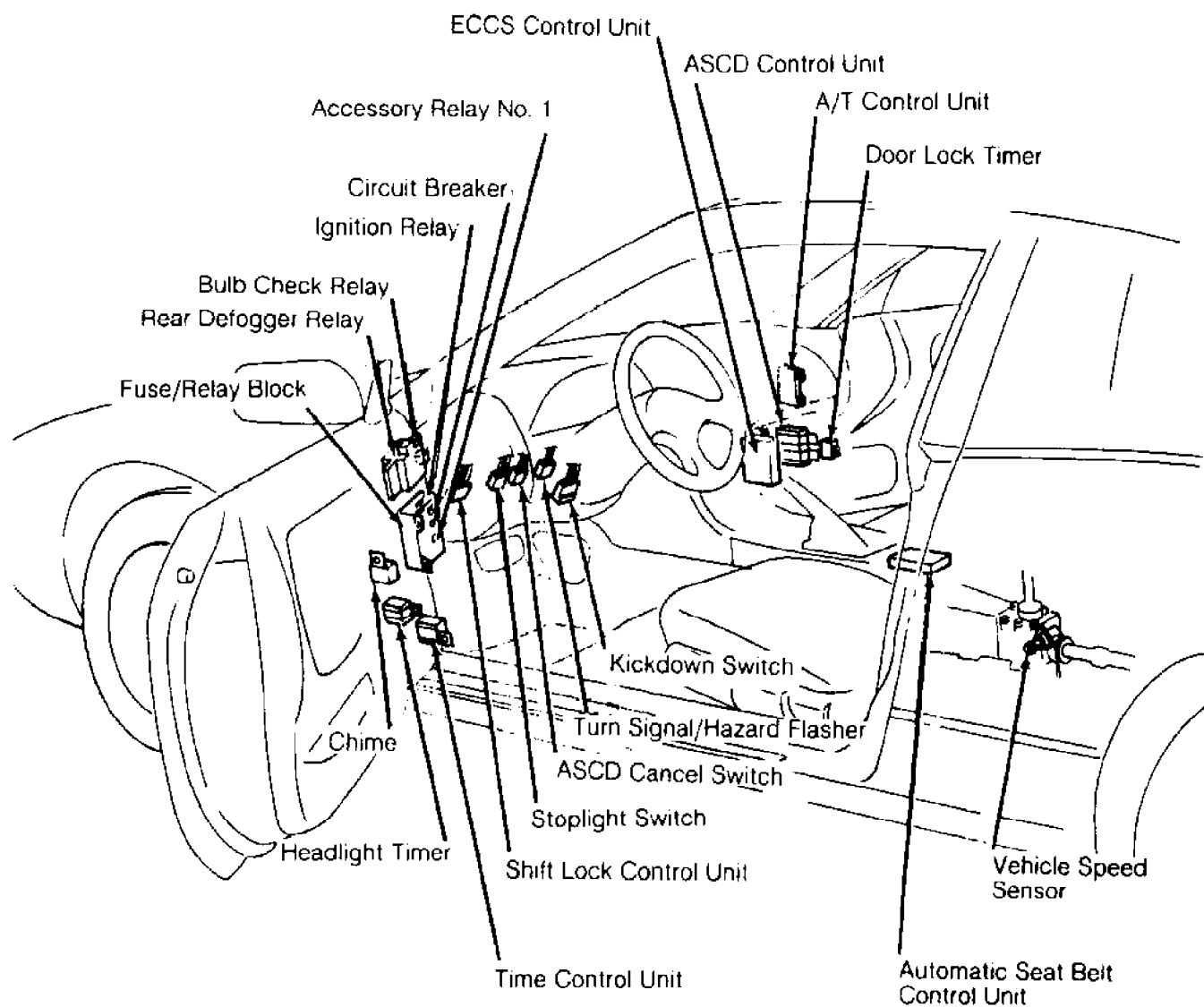
Electronic Concentrated Control System (ECCS) Control Unit
