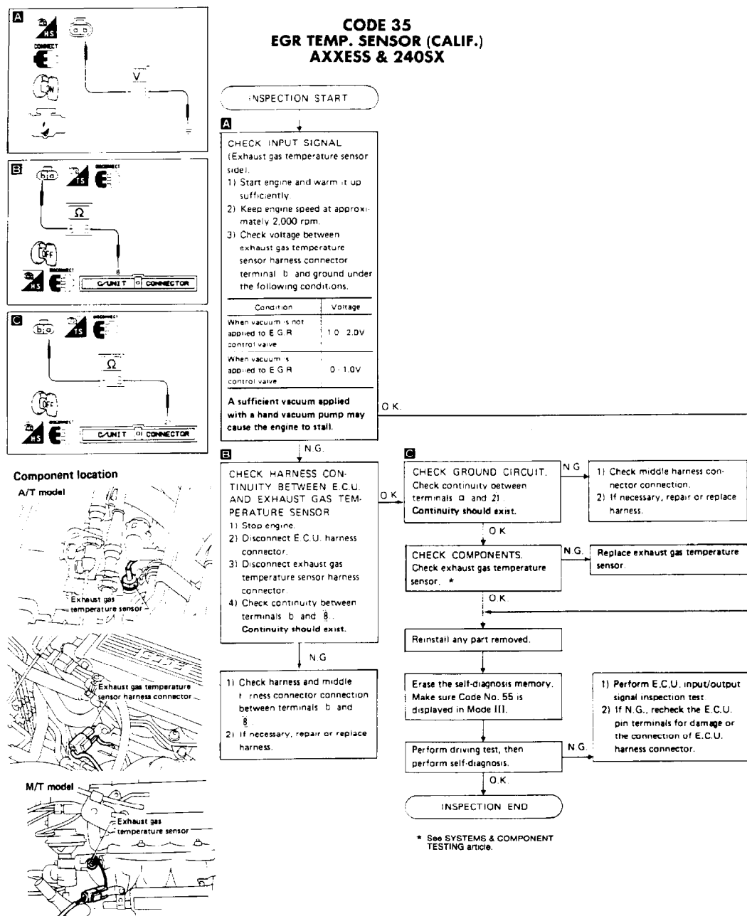
Fig. 13: Code 35: EGR Temp Sensor Test (Calif) Courtesy of Nissan Motor Co., U.S.A.
