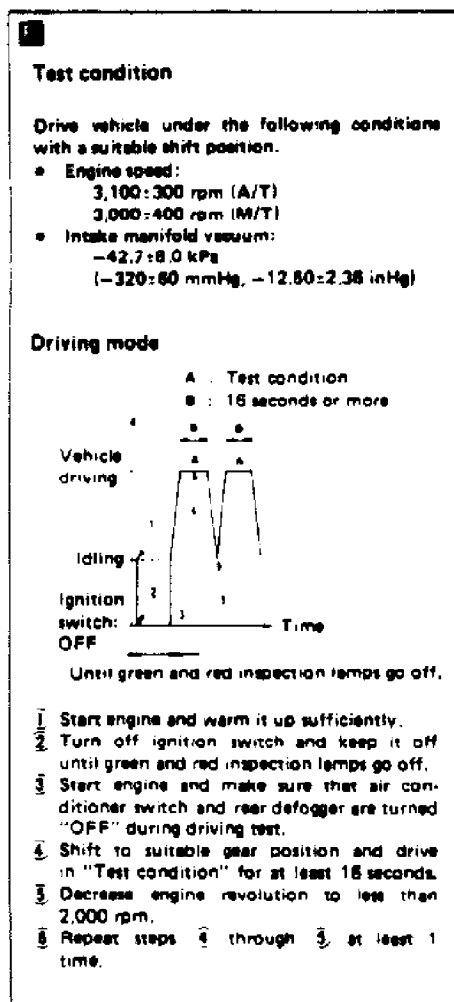
Fig. 9: Code 32: EGR Sensor 240SX (Calif) (2 of 2) Courtesy of Nissan Motor Co., U.S.A.
