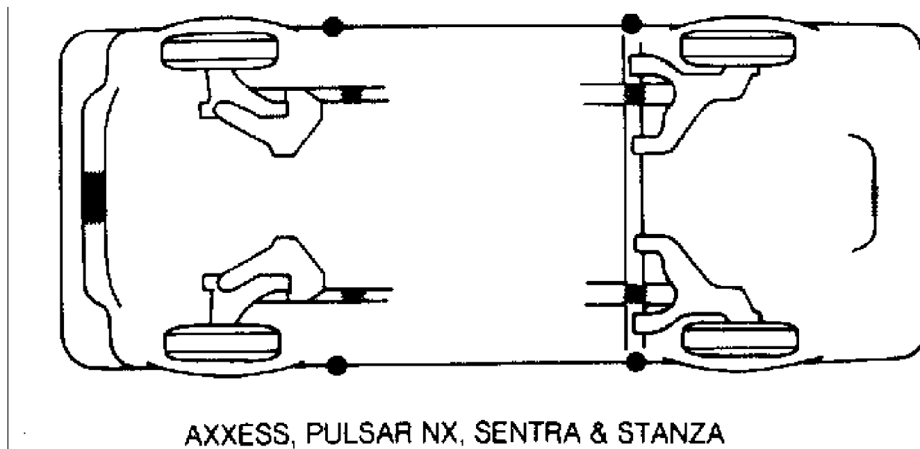
Fig. 1: Vehicle Frame, Underbody & Outerbody Lifting Points (Axxess, Pulsar, Sentra, Stanza) Courtesy of Nissan Motor Co., U.S.A
