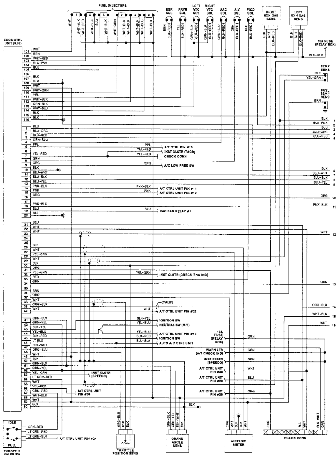
Fig. 10: 300ZX 3.0L Wiring Diagram (1 of 2)
