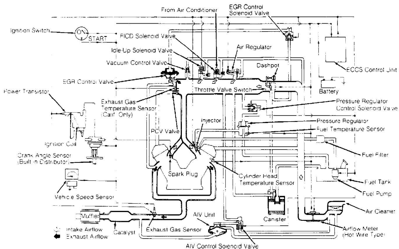
Fig. 10: 300ZX Vacuum Diagram Courtesy of Nissan Motor Co., U.S.A.
