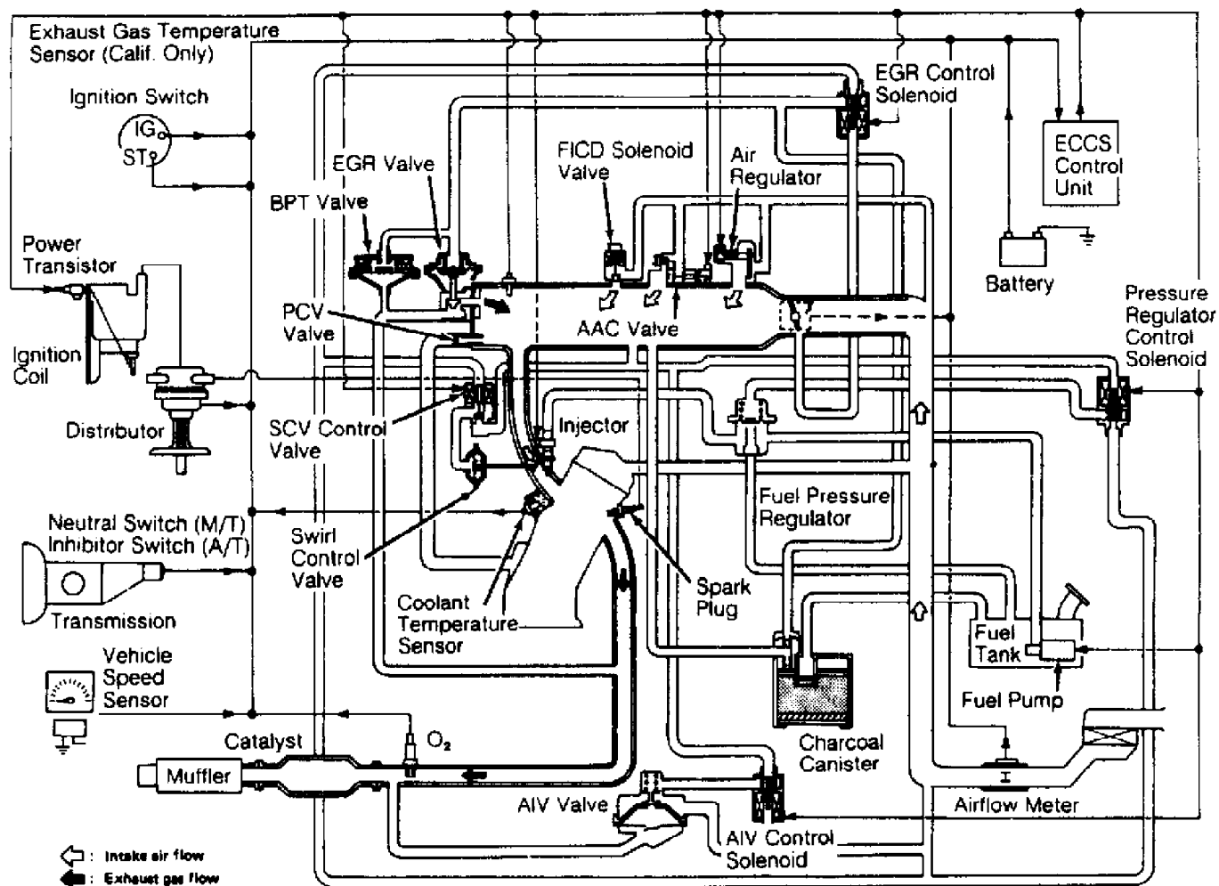
Fig. 9: 240SX Vacuum Diagram Courtesy of Nissan Motor Co., U.S.A.
