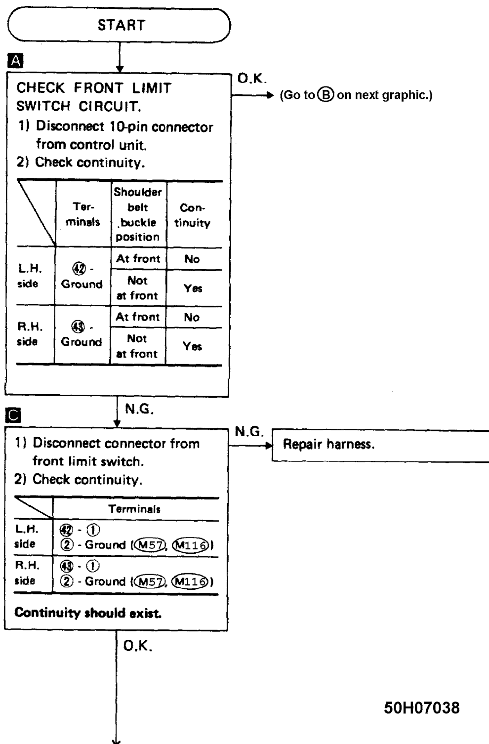
Fig. 23: Diagnostic Procedure 3 (1 of 2)
