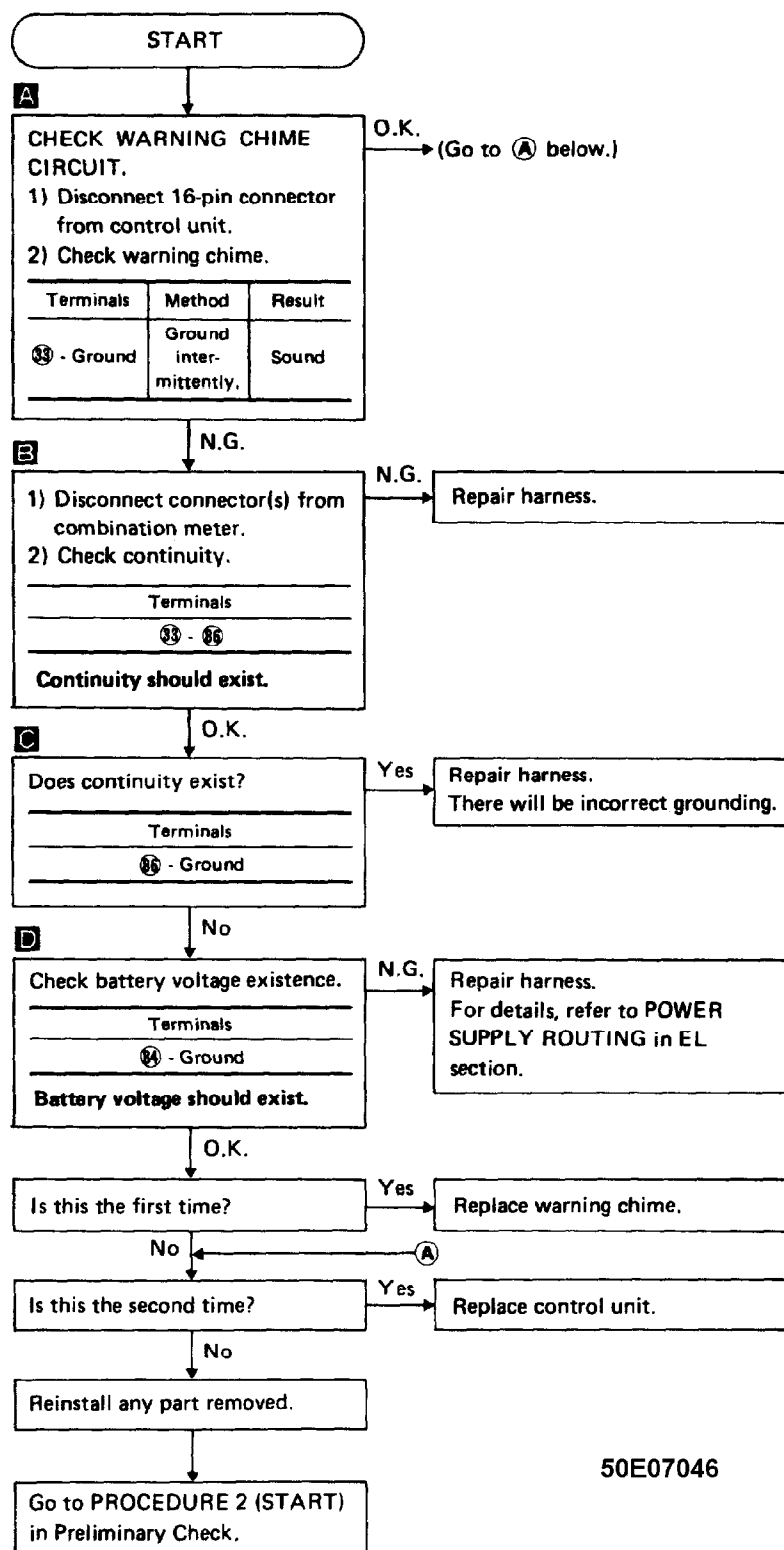
Fig. 31: Diagnostic Procedure 7
