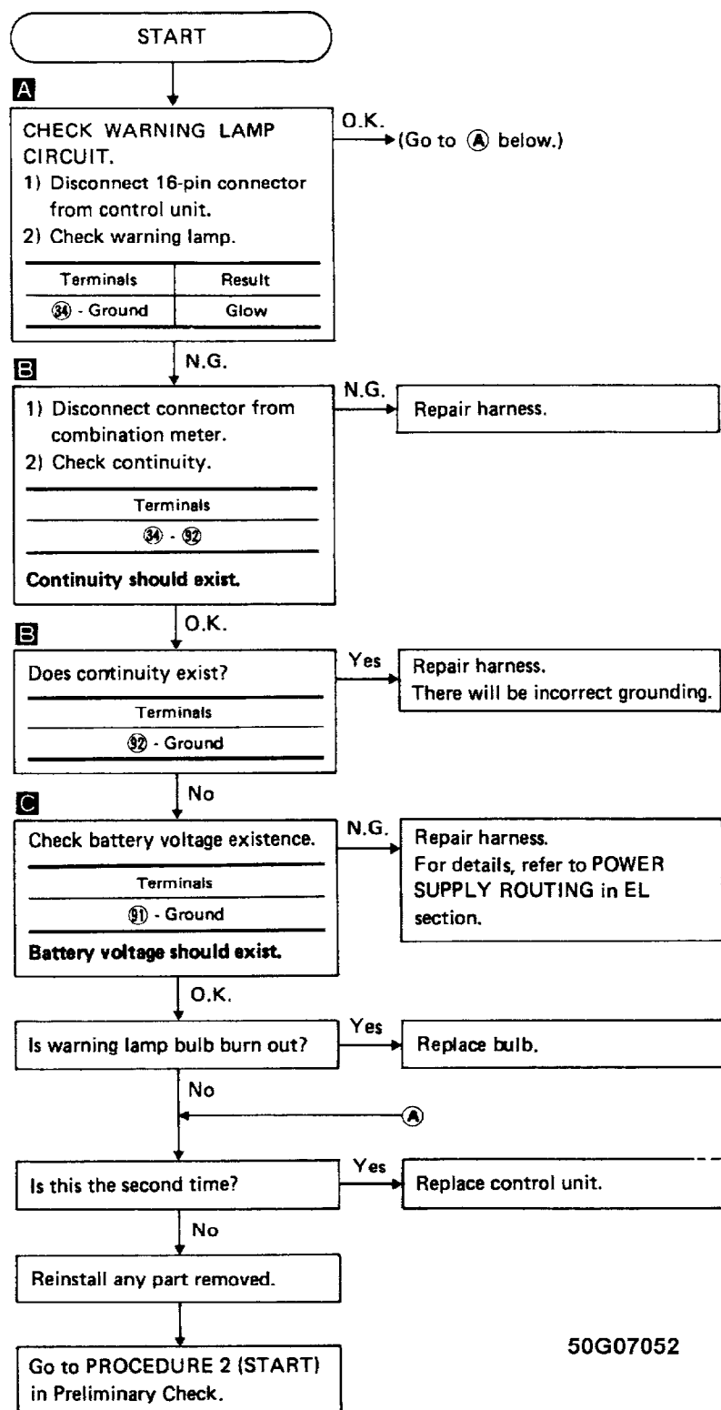
Fig. 32: Diagnostic Procedure 8
