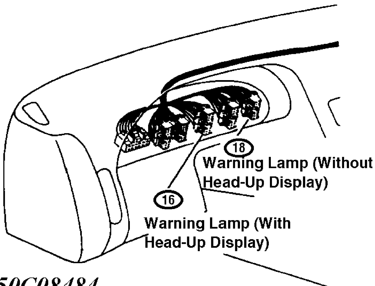
Fig. 4: Warning Lamp
