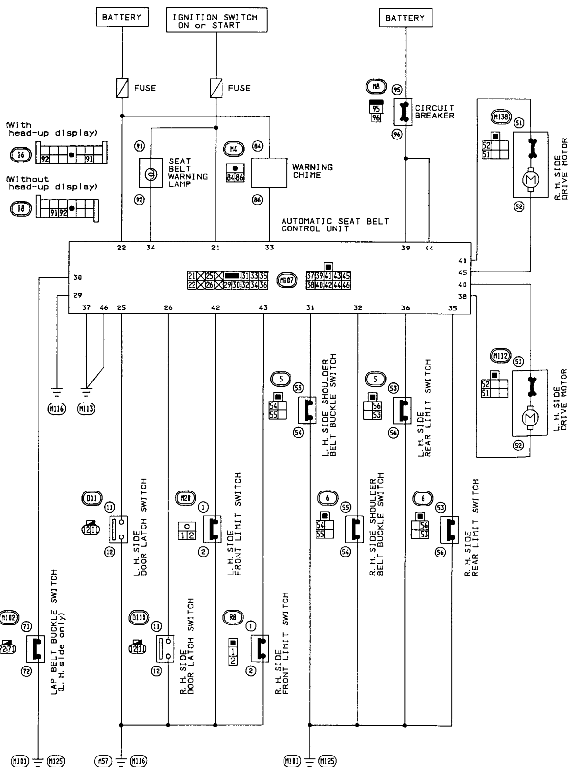
Fig. 8: Quick Pinpoint Check Circuit Diagram
