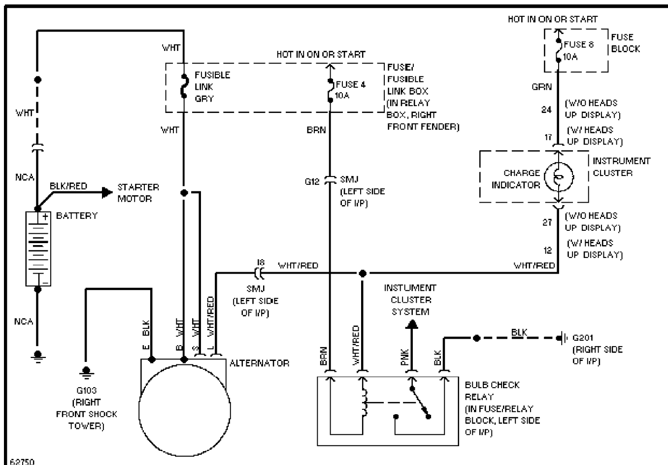
62750 Charging Circuit
