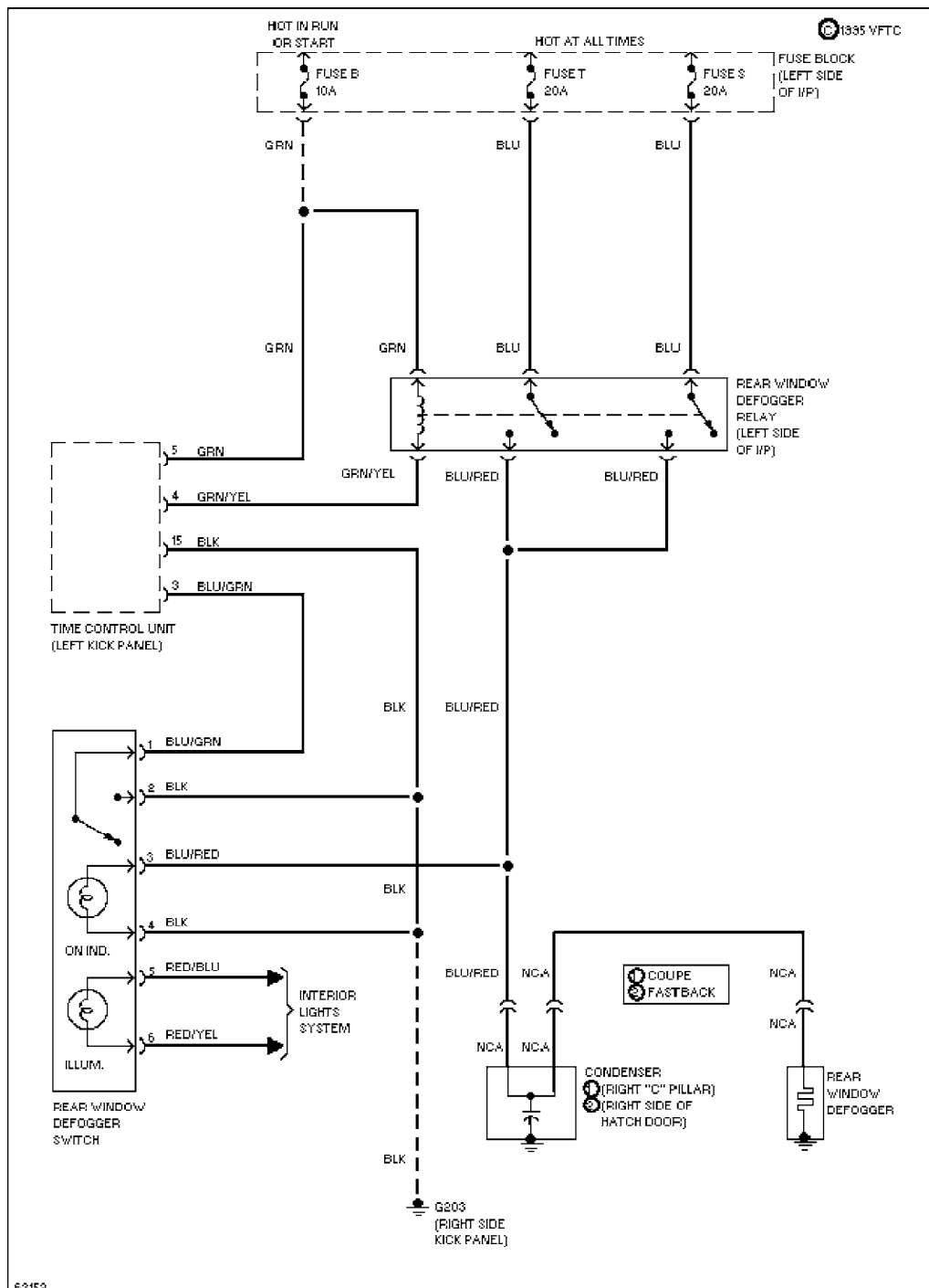
Defogger Circuit
