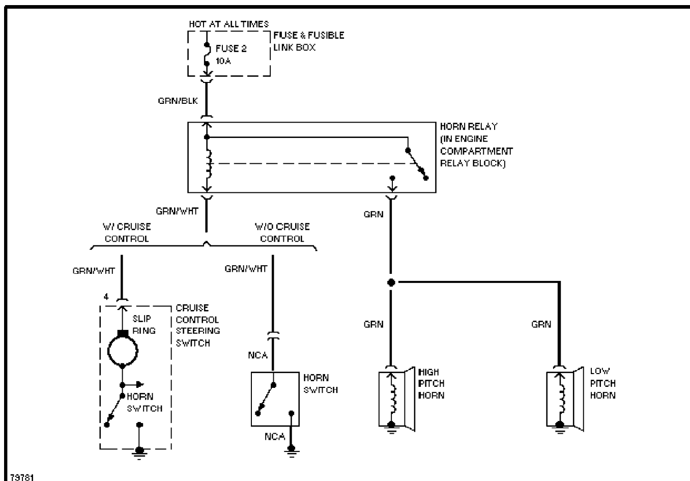
Horn Circuit
