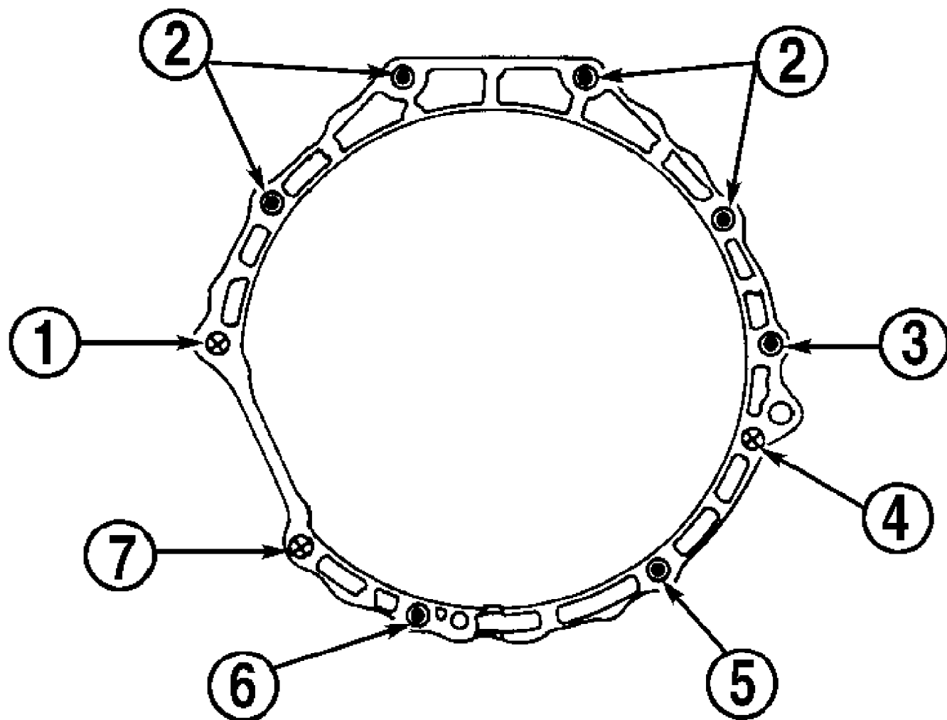
Fig. 1: Tightening Sequence For Engine-To-Transmission Bolts (300ZX) Courtesy of Nissan Motor Co., U.S.A.
