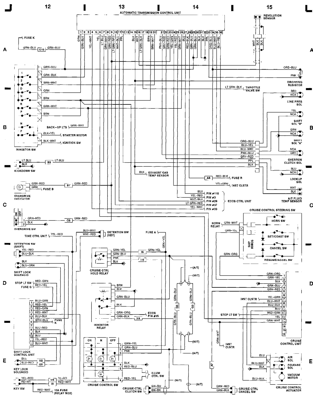
Fig. 4: Elect A/T Control, Cruise Control (Grids 12-15)
