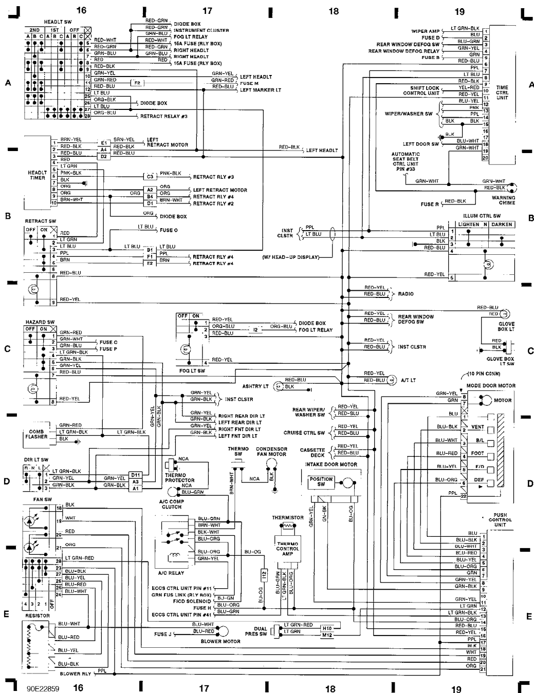
Fig. 5: A/C & Heater, Steering Column (Grids 16-19)
