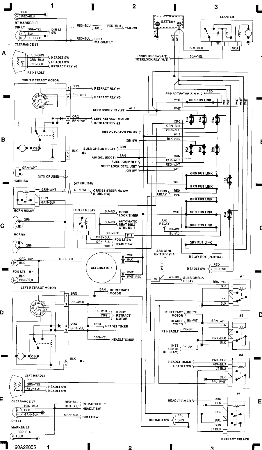
Fig. 1: Engine Compartment & Headlights (Grids 1-3)
