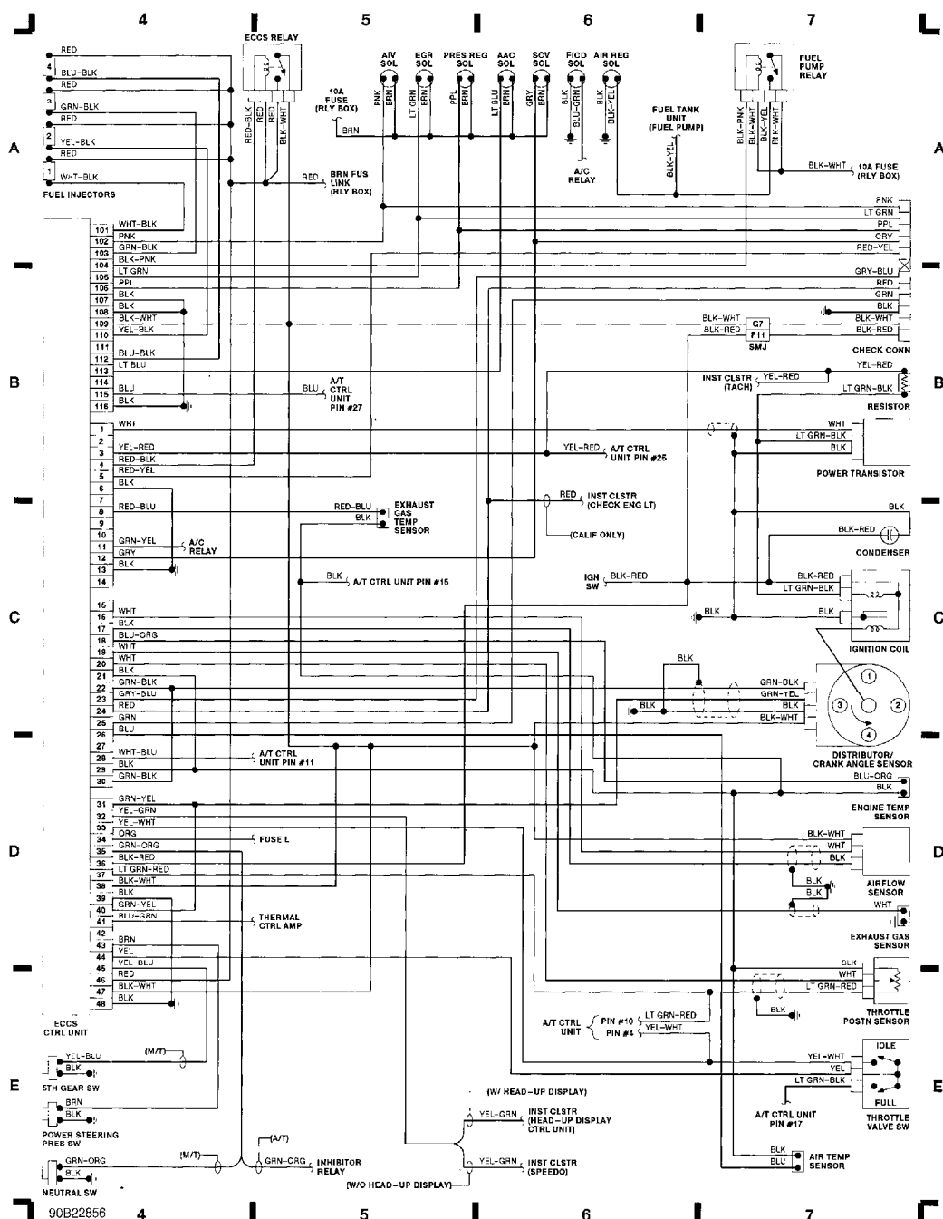
Fig. 2: Computer Engine Control (Grids 4-7)
