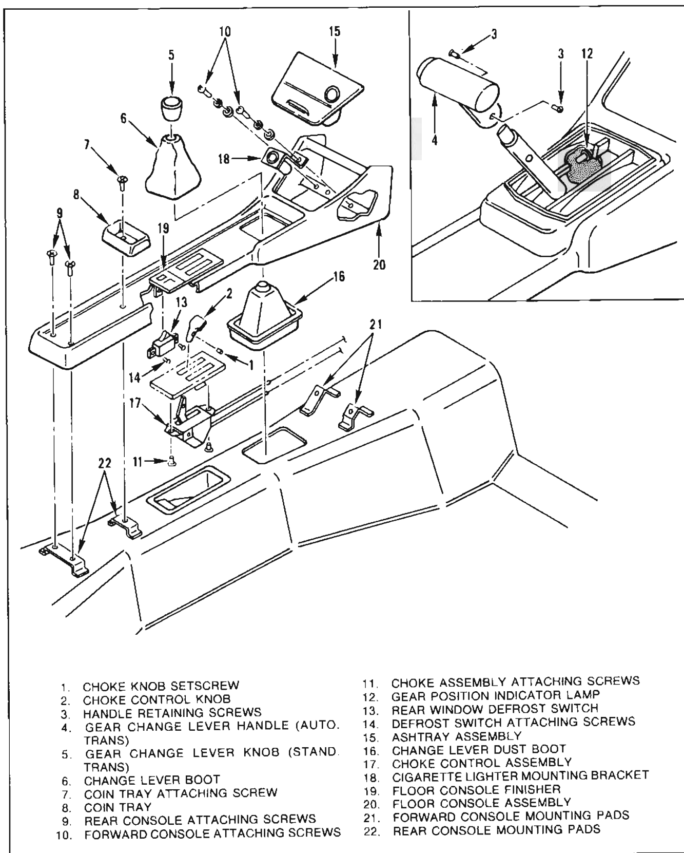
Figure II-1. Floor Console and Attaching Hardware (Exploded View)
