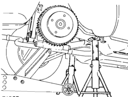
Fig. GI-9 Rear supportable point
