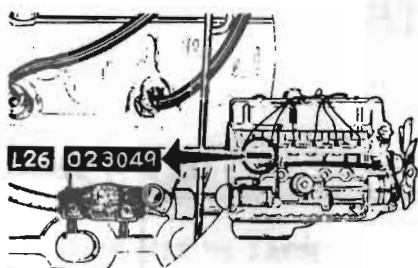
Fig. GI-3 Engine serial number location
