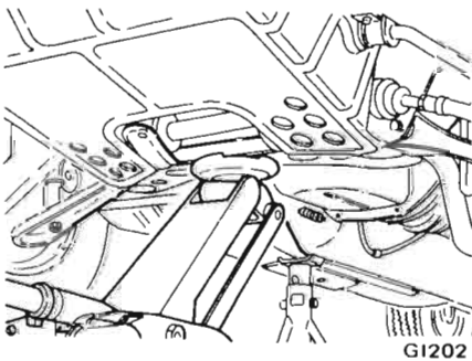
Fig. GI-6 Front jacking point
