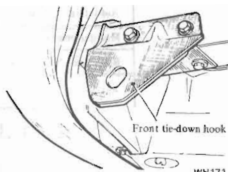
Fig. GI-11 Front tie-down hook
