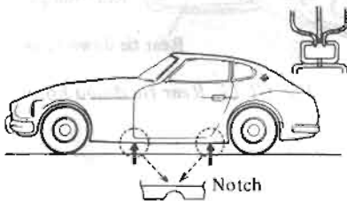
GI201 Fig. G1-5 Jacking point
