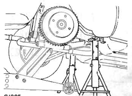
Fig. G1-9 Rear supportable points
