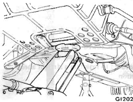
Fig. G1-6 Front jacking point
