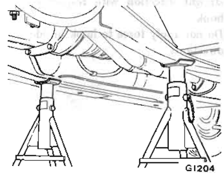
Fig. G1-8 Front supportable points
