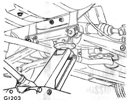
Fig. G1-7 Rear jacking point
