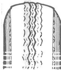
Underinflation wear
