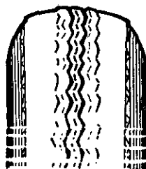
Underinflation wear
