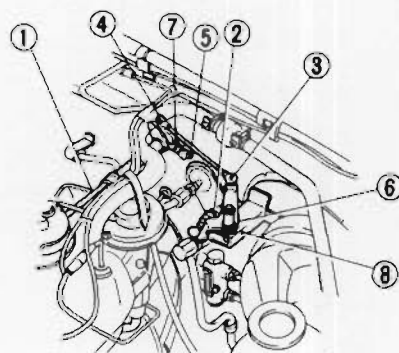
Fig. FE-1 Accelerator linkage
