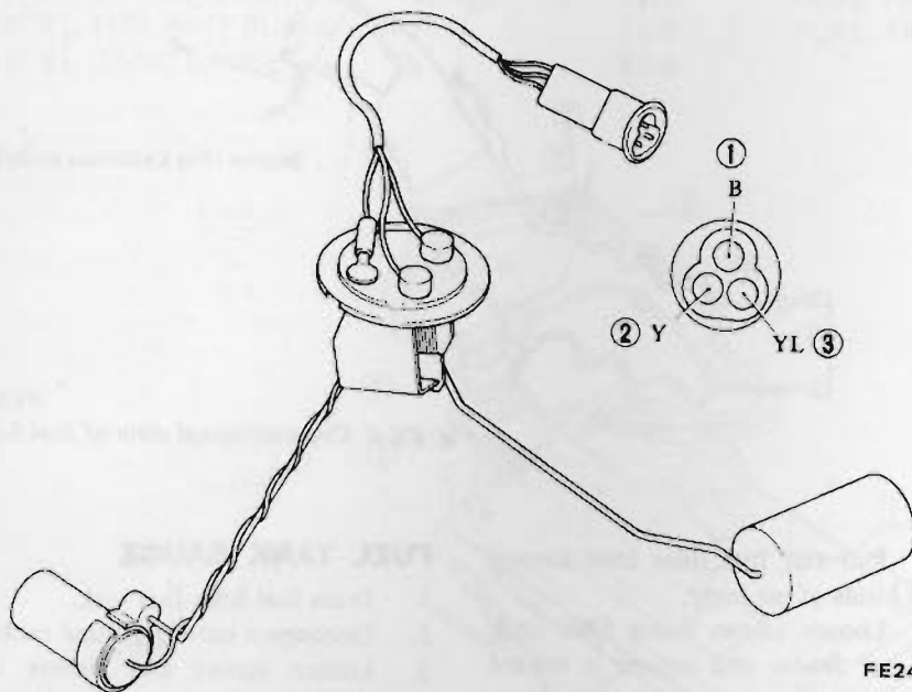
Fig. FE-10 Fuel tank gauge
