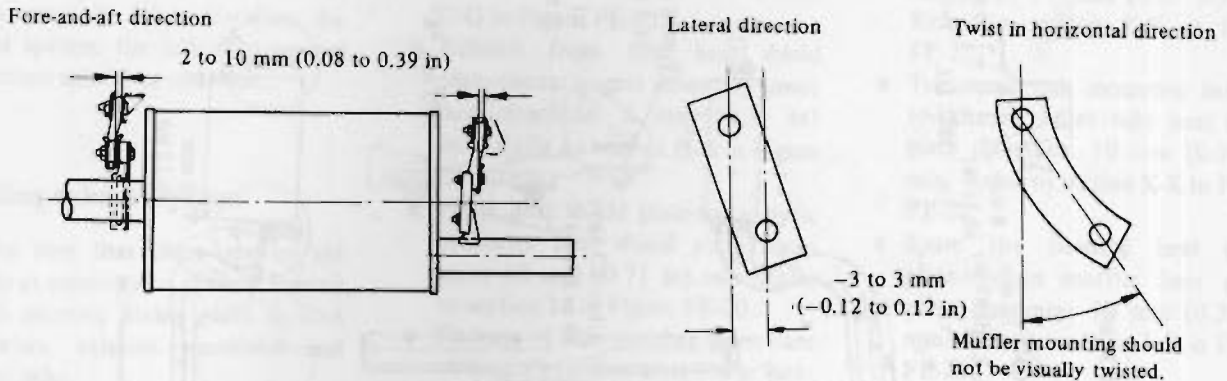
Fig. FE-21 Mounting rubbers
