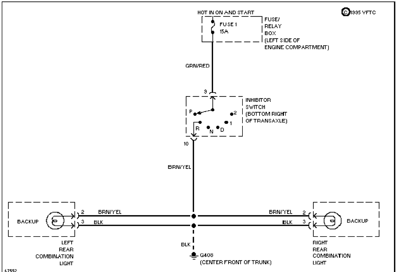
67552 Back-up Lamps Circuit
