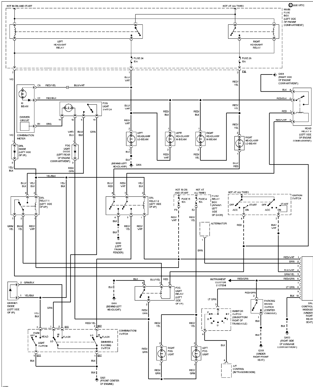
Headlight Circuit, W/ DRL
