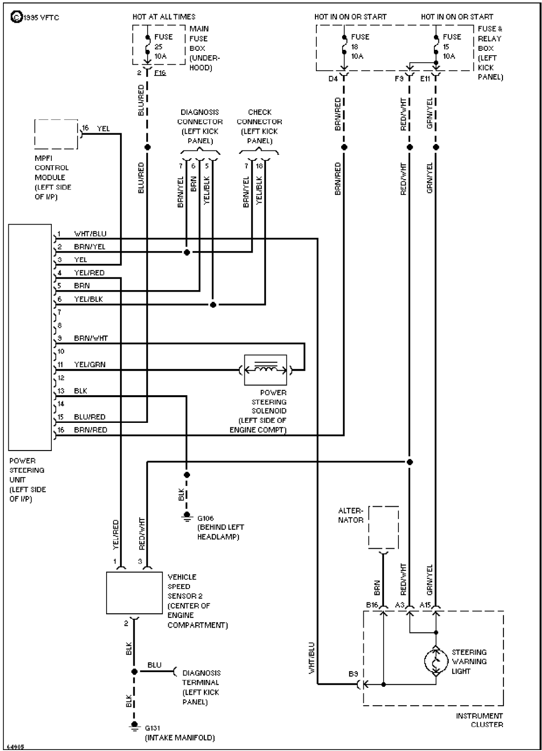
Electronic Power Steering Circuit
