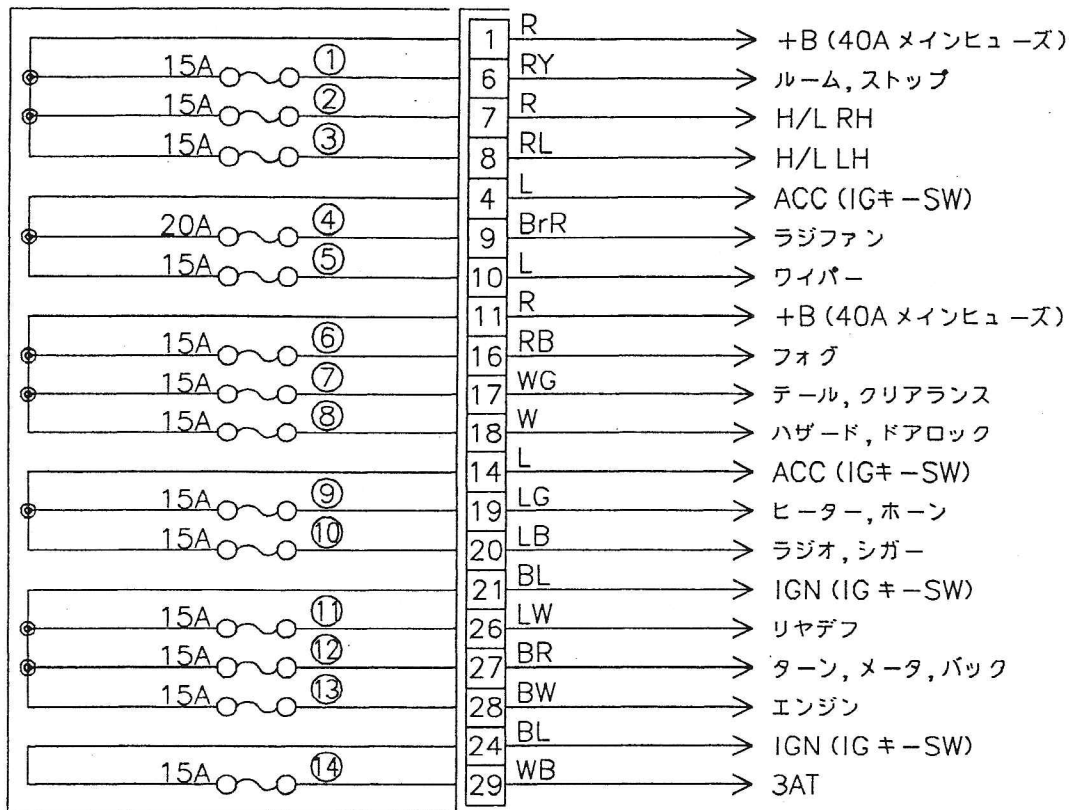
1 (FUSE BLOCK)
