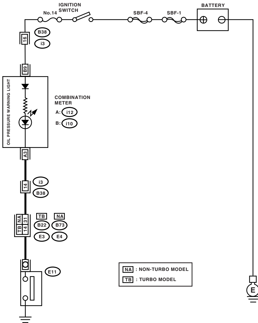
OIL PRESSURE SWITCH
