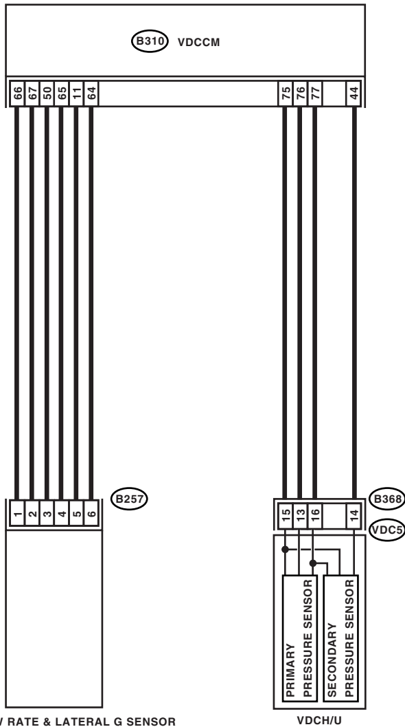
YAW RATE & LATERAL G SENSOR
