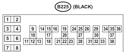
RELAY BLOCK
