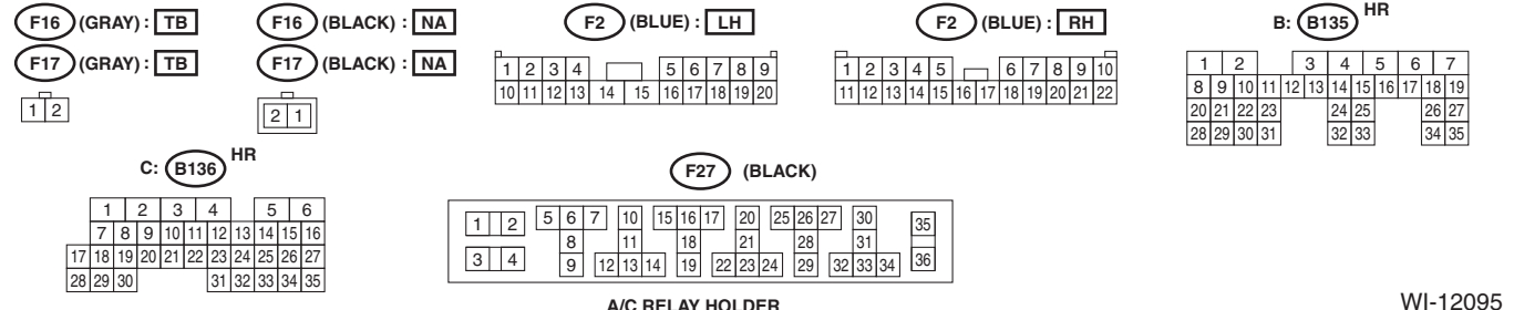
A/C RELAY HOLDER
