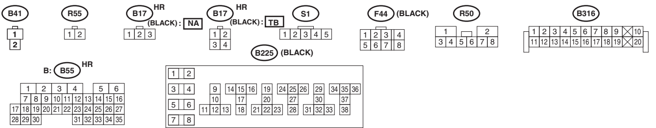
RELAY BLOCK
