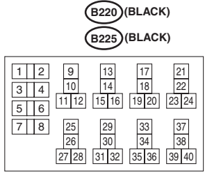
RELAY BLOCK
