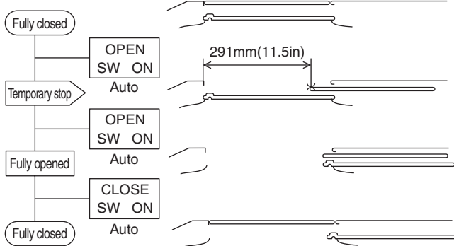
Open/close switch operation OUTBACK
