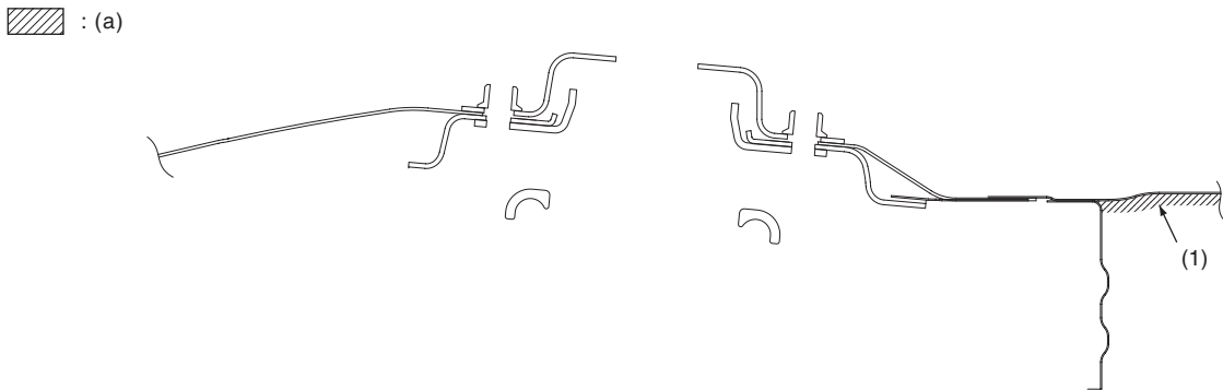
Cross section J — J
