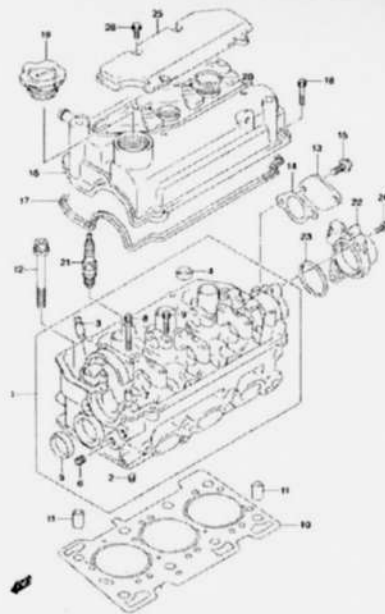
DAKIT 2 303 CYLINDER HEAD (4V)
