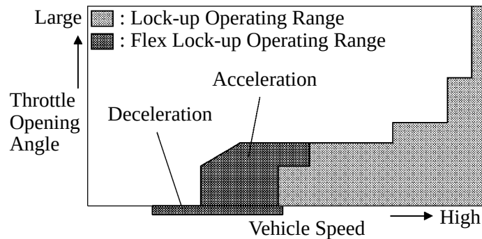
Flex Lock-up Operating Range
