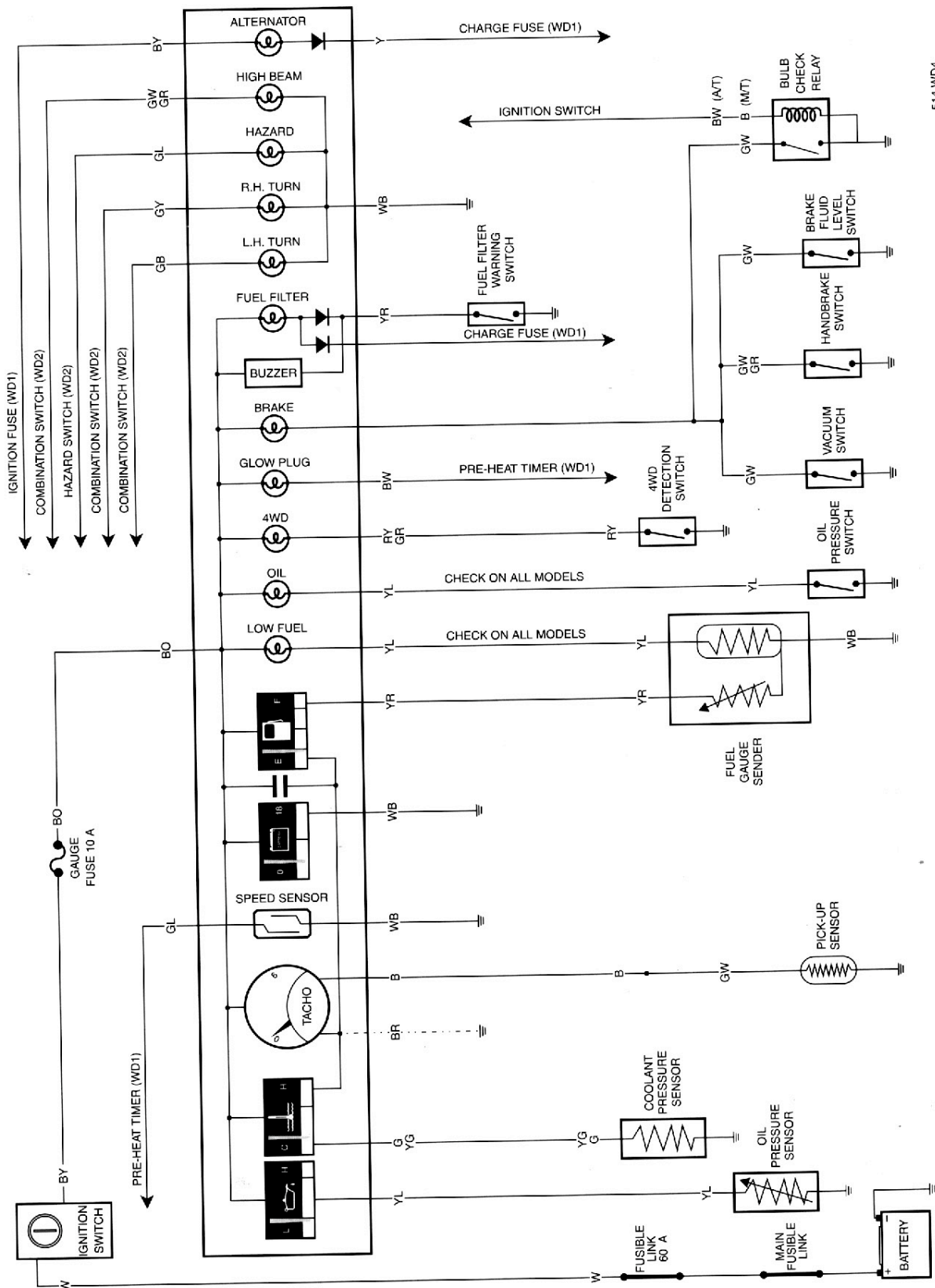
Instrument cluster.
