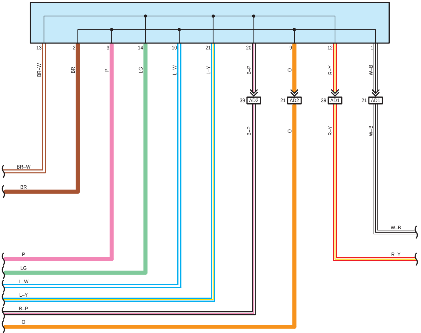
D43 Junction Connector
