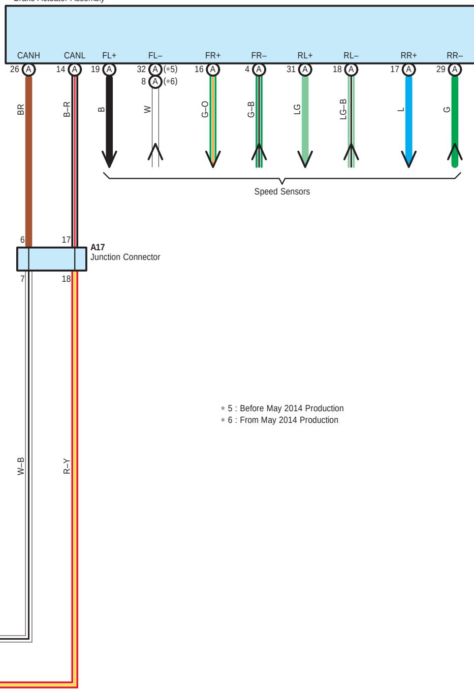
A5(A) Brake Actuator Assembly
