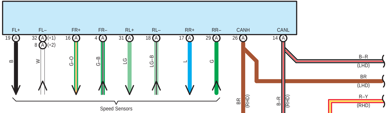
A5(A) Brake Actuator Assembly
